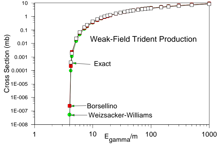
Figure 3: Calculated cross sections for the trident process (1) for the initial electron at rest and initial photon of energy E_\gamma . Then E_\gamma/m = (s - s_{\min})/2m^2 , the invariant measure of the energy of the interaction above threshold.
