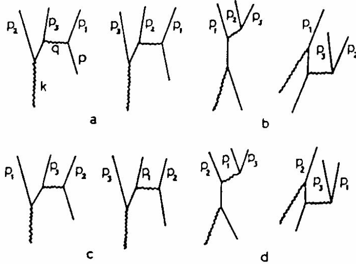
Figure 2: Feynman diagrams for reaction (1). Diagrams (b) and (d) are called \gamma - e or Compton diagrams.
