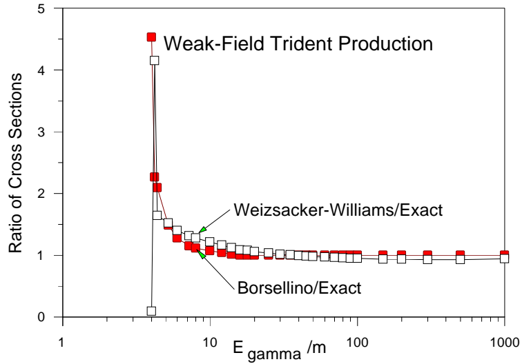
Figure 4: Ratio of calculated cross sections of the trident process (1).
