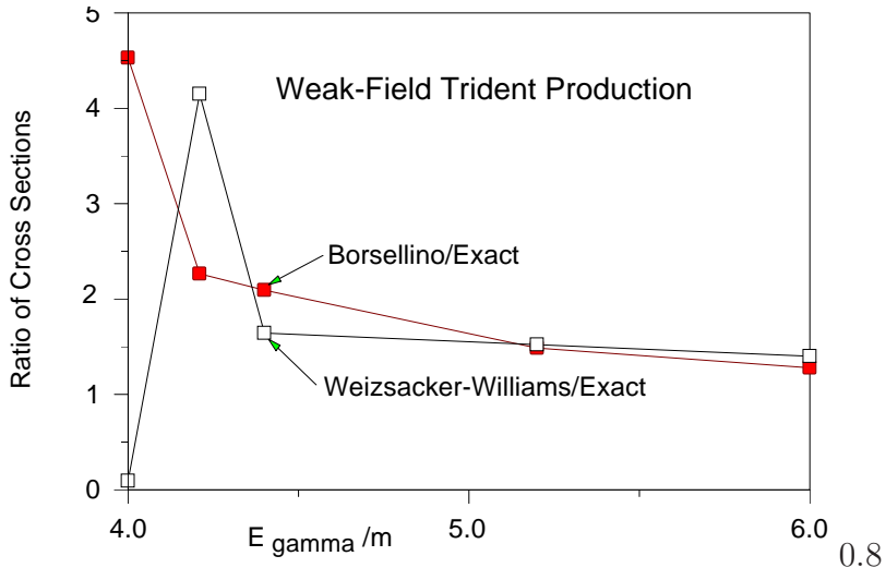
Figure 5: Ratio of calculated cross sections of the trident process (1).
