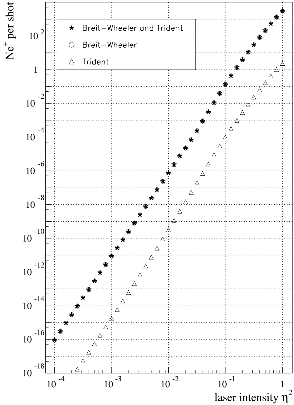
Figure 8: Calculated rates for trident production (16) and two-step pair creation (23) for typical conditions of our experiment [4].
