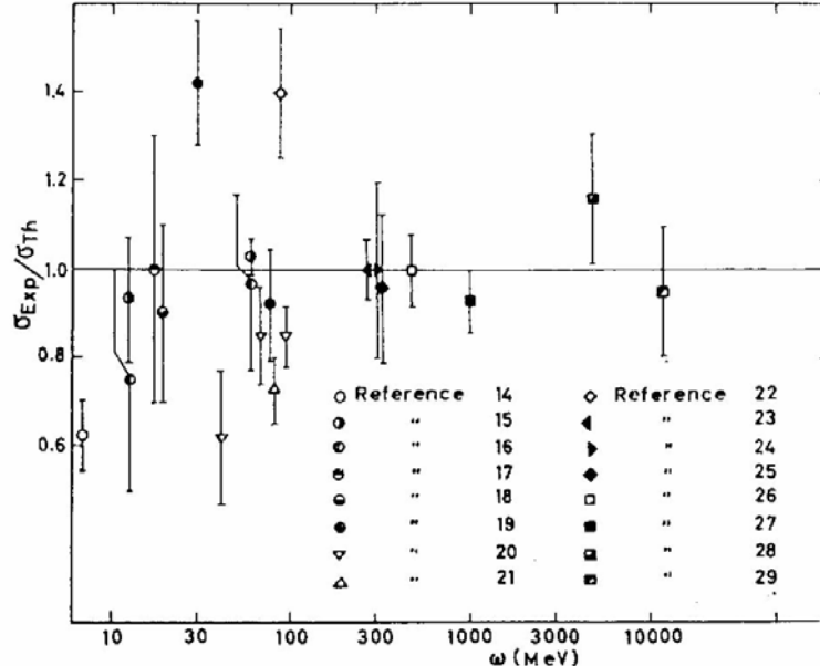
Figure 1: Comparison of theory and experiment for reaction (1). From [5], which includes references to the experiments.
