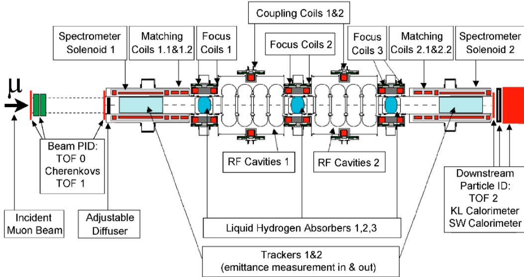
Fig. 10: Schematic drawing of MICE apparatus, comprising a muon beam line at left (not shown), particle-identification systems, and input and output spectrometers surrounding a single ionization-cooling lattice cell.
