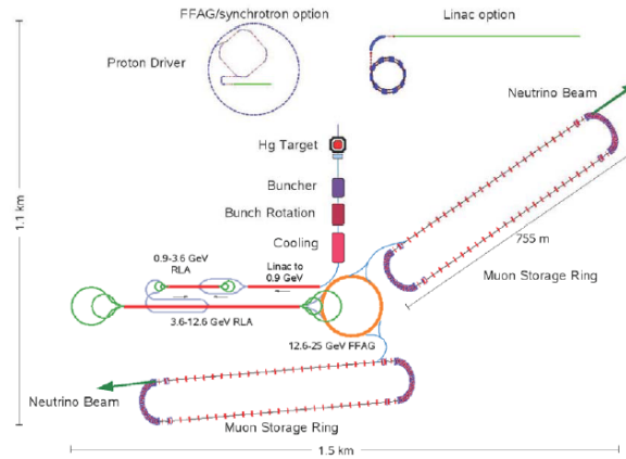
Fig. 6. Diagram of the IDS-NF baseline NF configuration.
