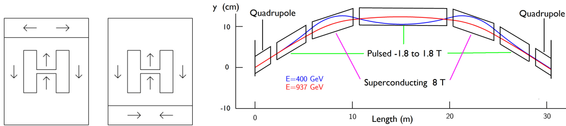
Fig. 9. Left: Alternating dipole laminations. Arrows show B field and grain direction. Right: Half-cell with interleaved fixed superconducting and fast ramping dipoles.
