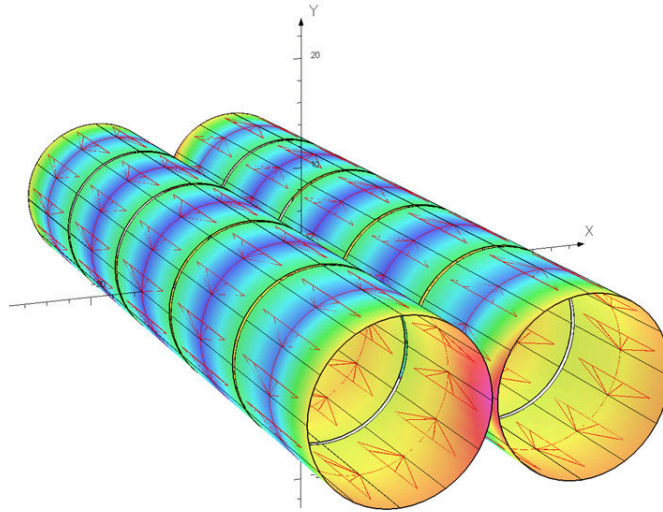
Fig. A-7. Magnetic cavern configuration.
