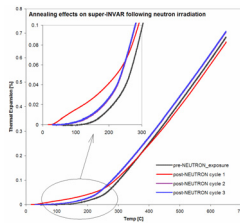
Figure 12: Damage reversal or CTE restoration in super-Invar following a third, neutron-dominated irradiation
