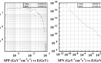
Figure 7: Estimated proton and neutron energy spectra
