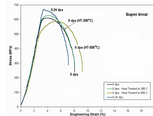
Figure 9: Proton irradiation effects and temperature effects on the stress-strain relation of super-Invar
