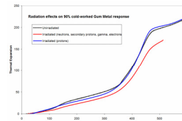
Figure 15: Proton and neutron irradiation effect comparison on the thermal expansion of gum metal
