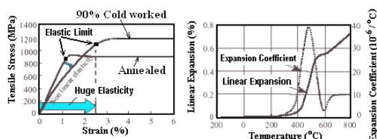
Figure 1: Un-irradiated Gum material properties [4]
