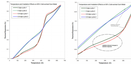
Figure 14: Proton irradiation and thermal effects on gum
