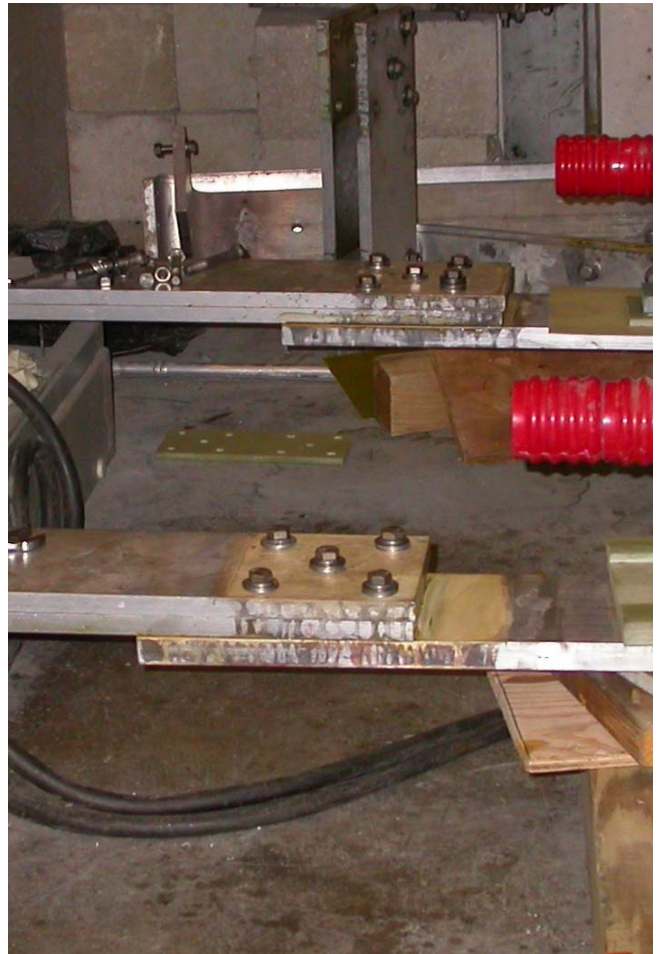
One end of Bus Bars Silver Plated and Bolted (not clamped)
