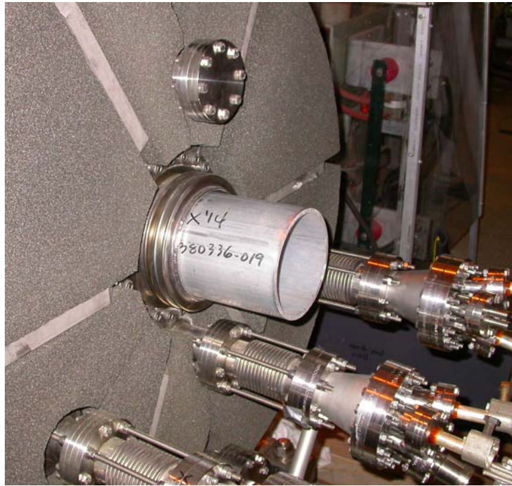
Go Gauge “Goes” at this end. Photo also shows foamglas insulation
