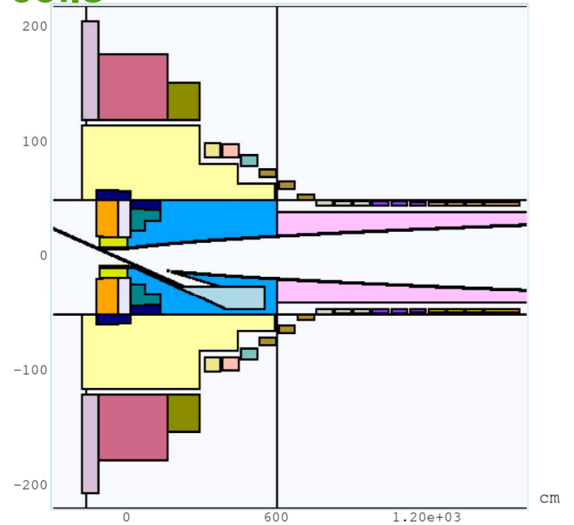
IDS120g with water cooling rings around RS coils
