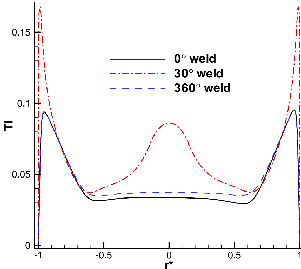
Horizontal line plot of turbulence intensity at the outlet of pipe
