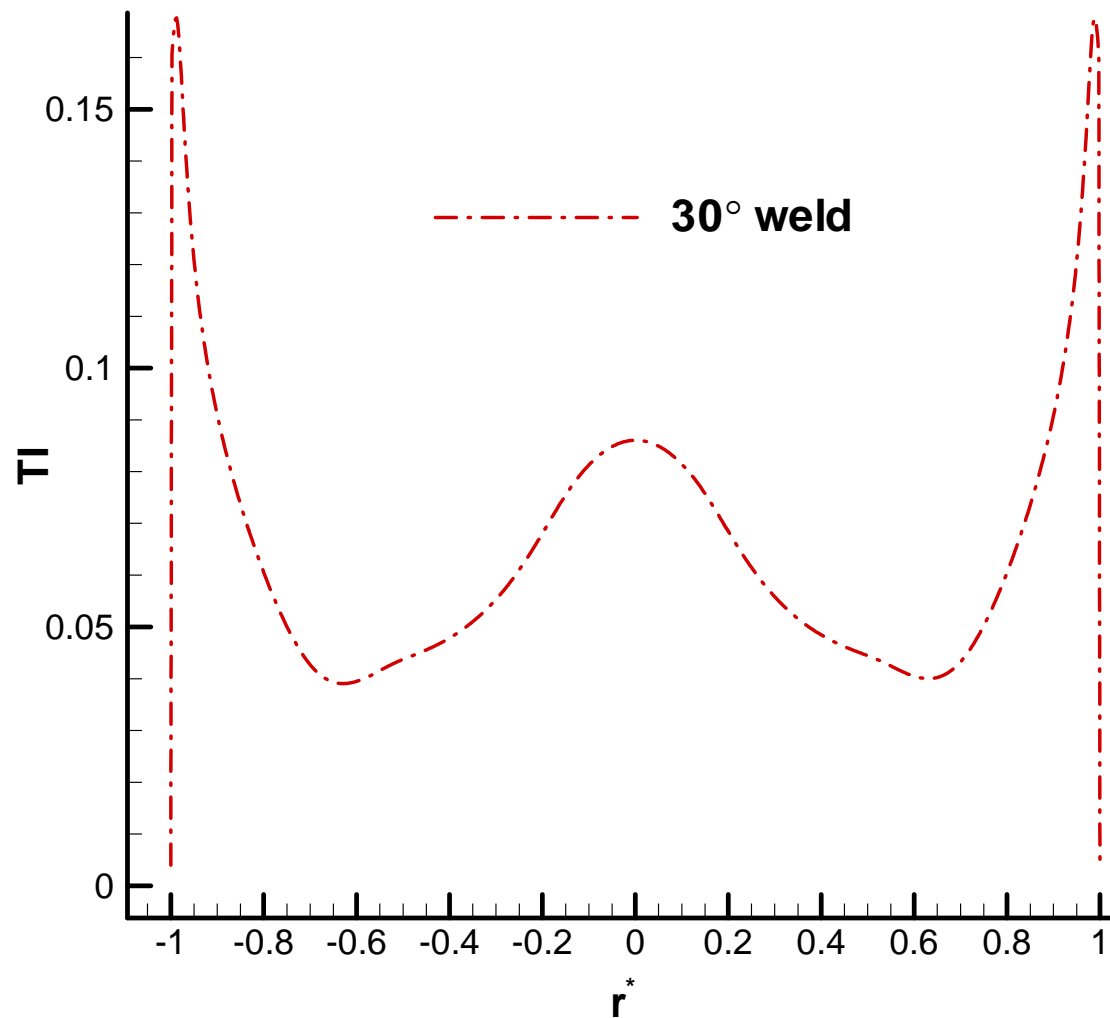
Vertical line plot of turbulence intensity at the outlet of pipe
