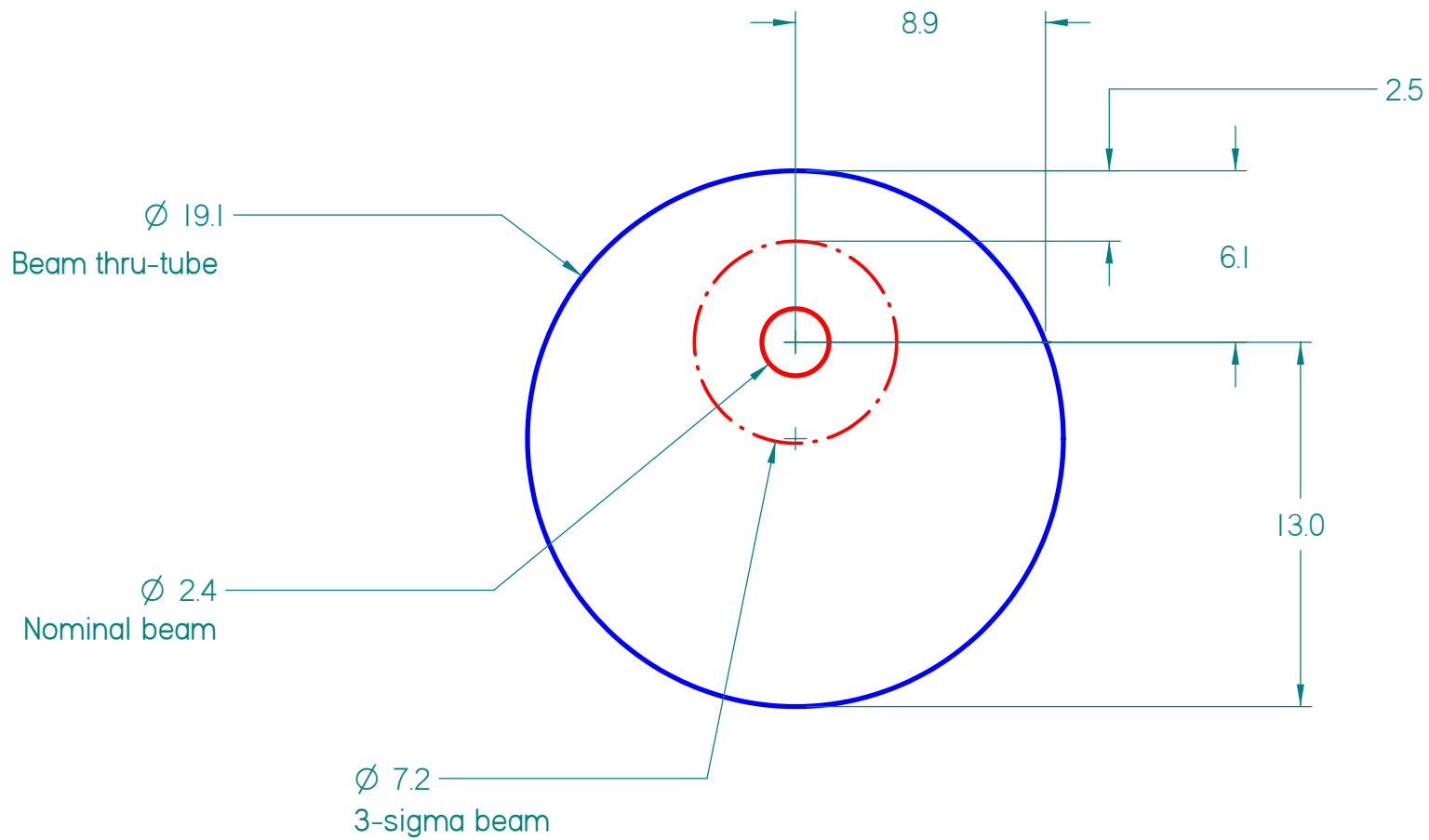
Beam Scanning Clearances in Primary Containment Nozzle Flange V.B. Graves 20 Dec 2005
