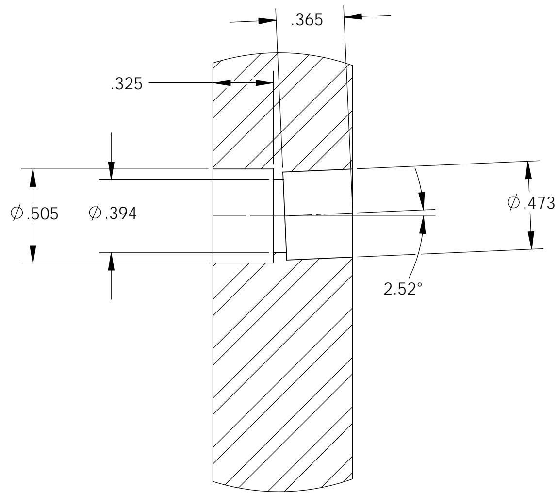
DETAIL B SCALE 2 : 1
