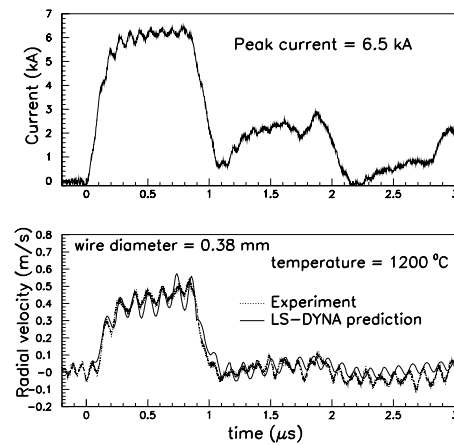
Figure 3: (Top) The current pulse shape for 6.5 kA peak current; (Bottom) Radial velocity of the 0.38 mm diameter tungsten wire at 1200 °C.
