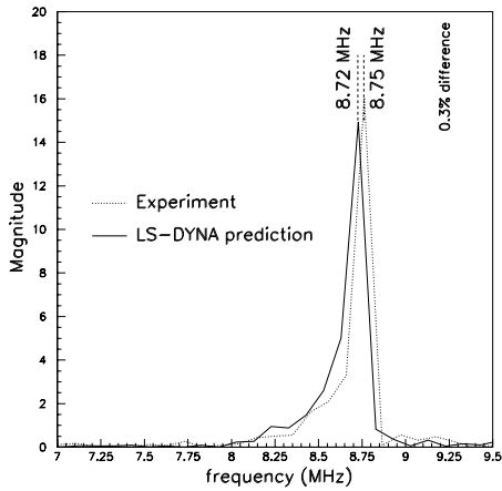
Figure 4: Measured and simulated characteristic frequency of radial vibrations of the 0.38 mm diameter wire measured at 1200 °C.
