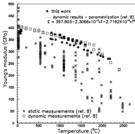
Figure 5: Comparison between our experimental results and previous results [8] on tungsten Young's modulus.
