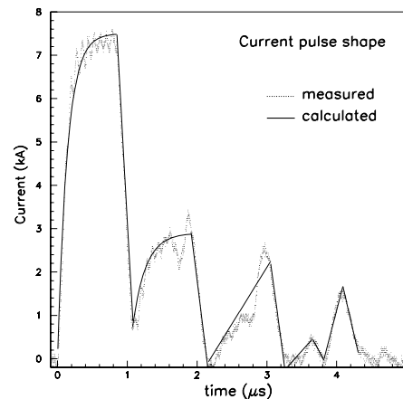
Figure 1: Measured and calculated (see text) waveform of the current pulse used in the experiment.
