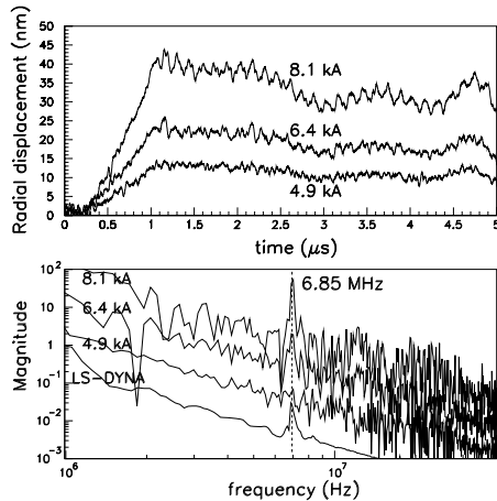
Figure 2: (Top) Radial displacement of the 0.5 mm wire as a function of applied current. (Bottom) Corresponding frequency spectra and the result of LS-DYNA prediction.
