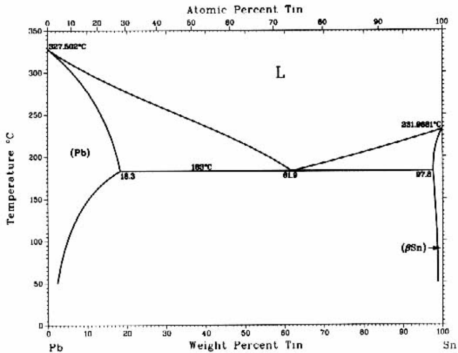
Figure 13: Pb-Sn phase diagram. Minimum melting temperature = 183°C.
