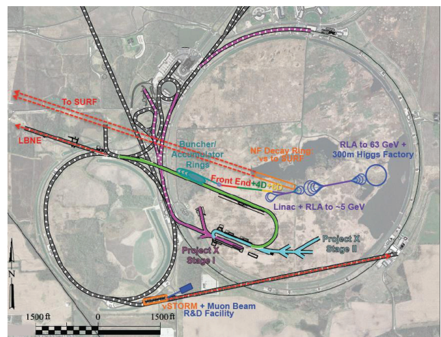
Figure 2: Footprint of Neutrino Factory and Higgs Factory Muon Collider facilities on the FNAL site.
