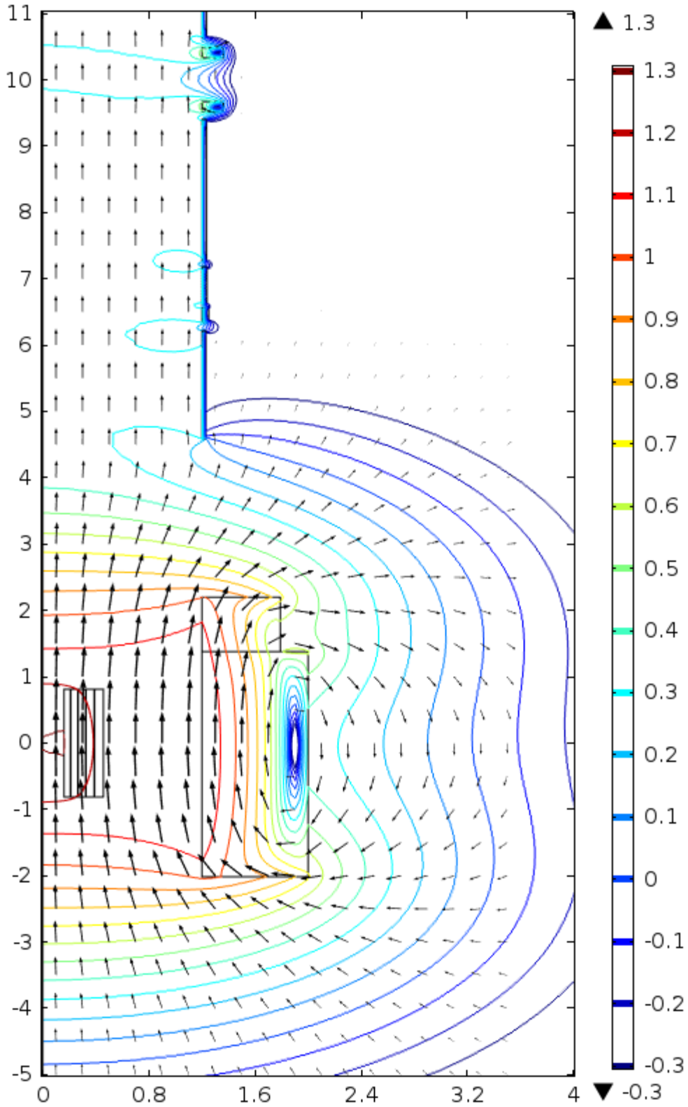
Fig. 1a Field direction (arrows) & \log_{10}|B| (contours) of Target Magnet "20to2T5m120cm4pDL"; consecutive contours are [ \sim 0.5 (navy), 0.63, 0.8, 1, 1.26, 1.6, 2.0, 2.5, 3.2, 4, 5, 6.3, 8, 10, 12.6, 16, 20 (maroon)] T.
