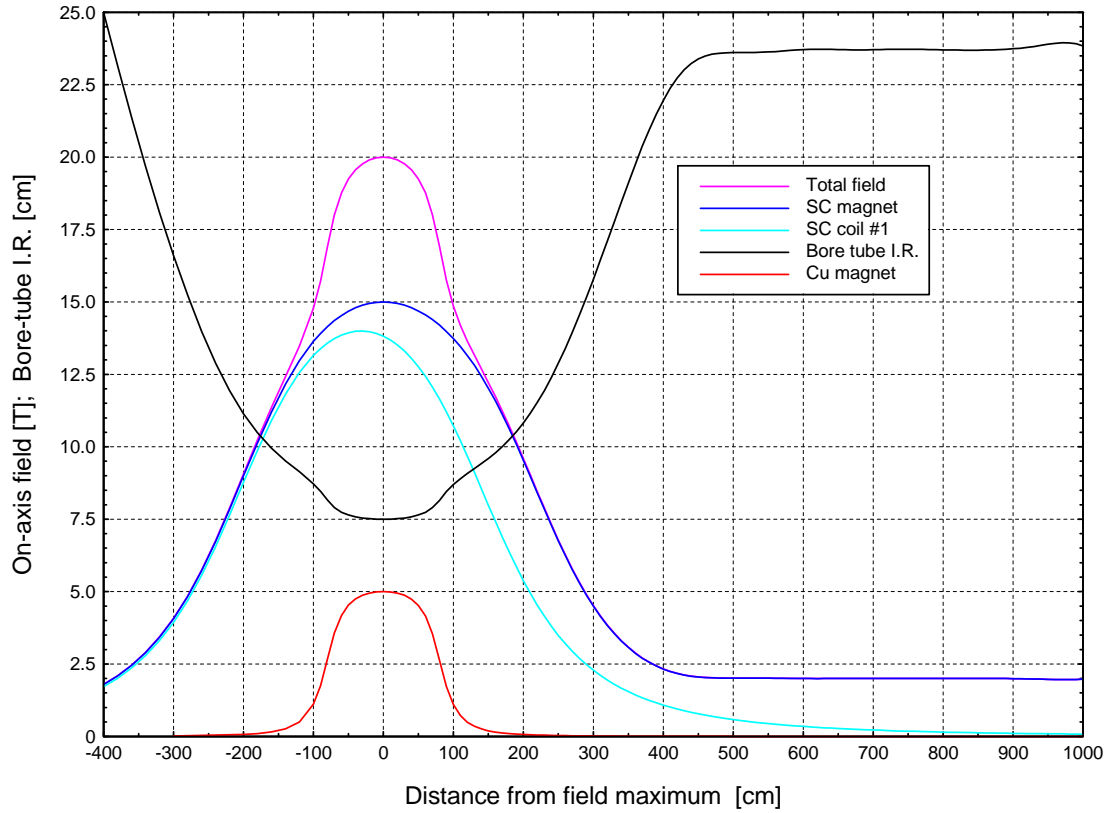
Target Magnet "20to2T5m120cm4pDL": Bore-Tube Radius and On-Axis Field Profiles
