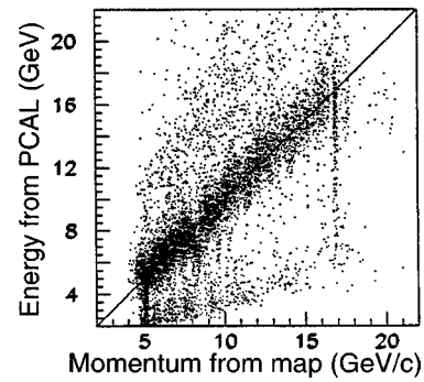
FIG. 21. The energy vs momentum of positrons observed in the PCAL from a calibration run with a 19-GeV electron beam incident on a foil in IP1.
