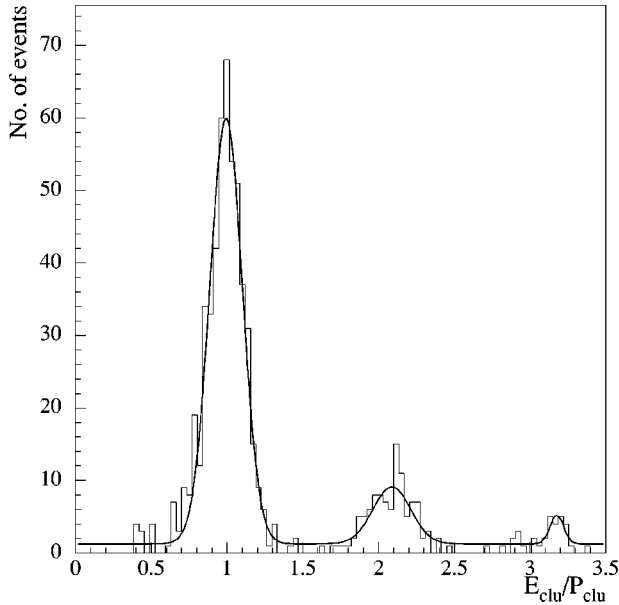
FIG. 32. Distribution of the ratio E_{\text{clu}}/P_{\text{clu}} for calibration clusters in PCAL row 7, which spans momenta from 20.3 to 21.5 GeV.
