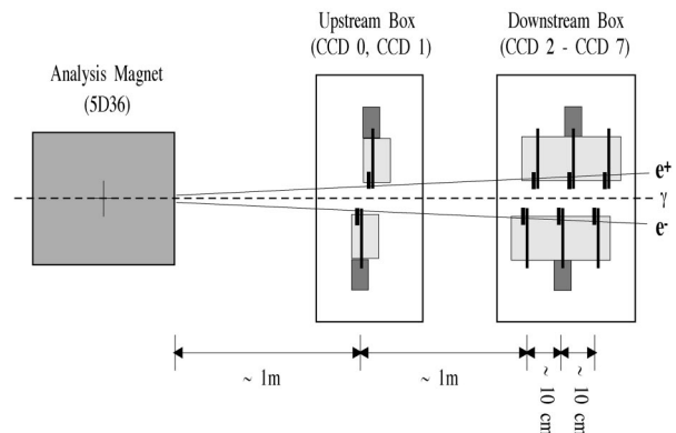
FIG. 22. Schematic of the CCD pair spectrometer.
