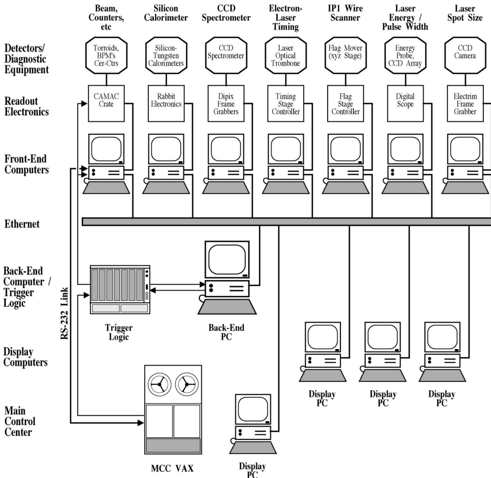
FIG. 25. Components of the data acquisition system.
