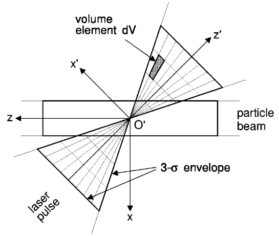
FIG. 52. Schematic of the integration grid along the x' axis and the z' axis. The variable size of the volume element dV as a function of z' is evident. For this example n_{x'}^\sigma = n_{z'}^\sigma = 3 and n_{x'}^\Delta = n_{z'}^\Delta = 8 .
