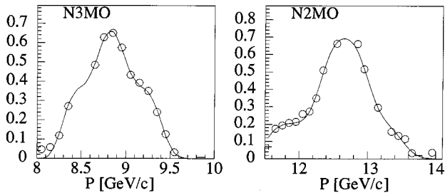
FIG. 24. Measured acceptances of electron detectors N2MO and N3MO vs electron momentum.
