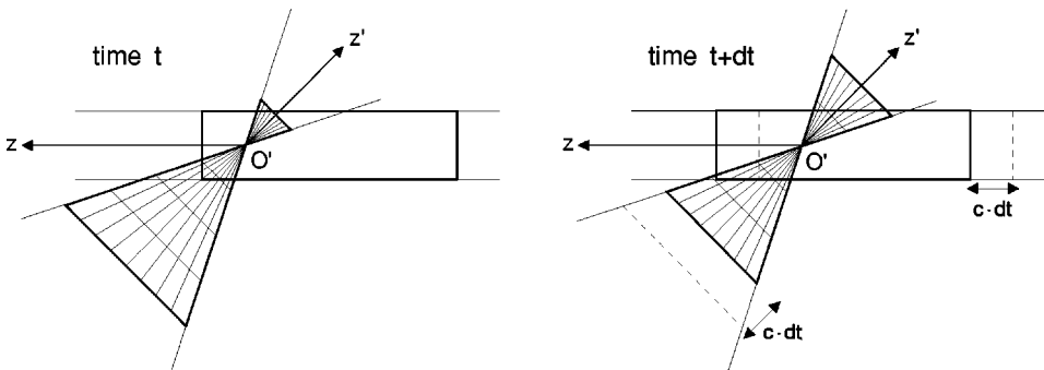
FIG. 53. The spatial integration grid at two consecutive time steps.
