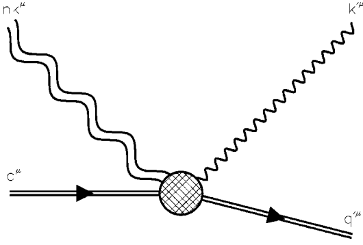
FIG. 6. Representation of nonlinear Compton scattering, process (1). An electron with quasimomentum q in a strong field (indicated by a double line) absorbs n photons (indicated by double sinusoids), emits a high-energy photon k' , and recoils with momentum q' .
