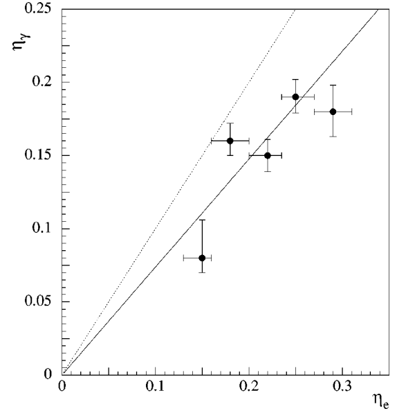
FIG. 41. Photon-based \eta_\gamma vs the mean value of the nonlinear-electron-based \eta_e for each of the five CCD data subsets. The vertical error bars are from the fit for \eta_\gamma using CCD data, and the horizontal error bars are the rms of the distribution of the monitor \eta_e .
