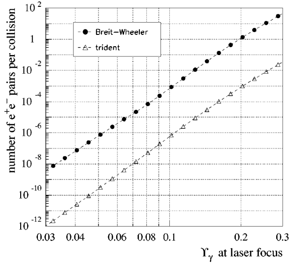
FIG. 10. The calculated rates for pair production from the multiphoton Breit-Wheeler process (2) and from trident production (53) as a function of Y_\gamma at the laser focus. In the present experiment, the maximum value of Y_\gamma was about 0.16.
