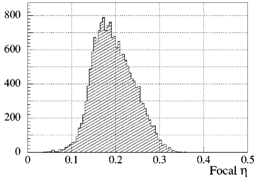
FIG. 37. Distribution of the laser field-strength parameter \eta calculated using the constrained fit (67) for the 46.6 GeV data with linearly polarized green light.
