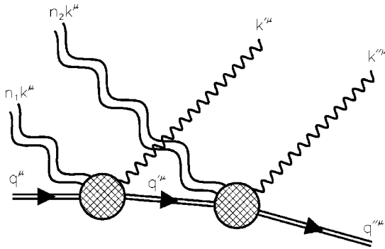
FIG. 7. Plural Compton scattering, process (38), of an electron in the laser field with n = n_1 + n_2 and m = 2 . The electron with initial momentum q scatters from n_1 laser photons, emitting a photon with momentum k' , and recoiling with momentum q' ; then the electron scatters again from the laser field, absorbing n_2 laser photons, emitting another photon k'' , and recoiling with momentum q'' .
