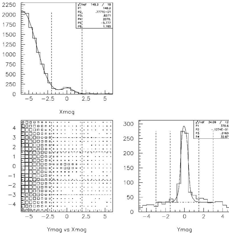
FIG. 31. The distribution of the track positions at the center plane of the magnet, using only high momentum electron tracks. Distances are in mm.
