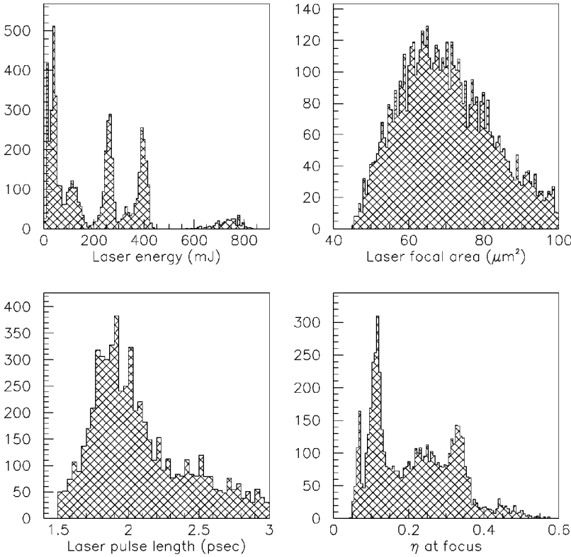
FIG. 28. Laser parameters for all data taken with IR pulses. The value of \eta at the laser focus was calculated by the direct method described in the text.
