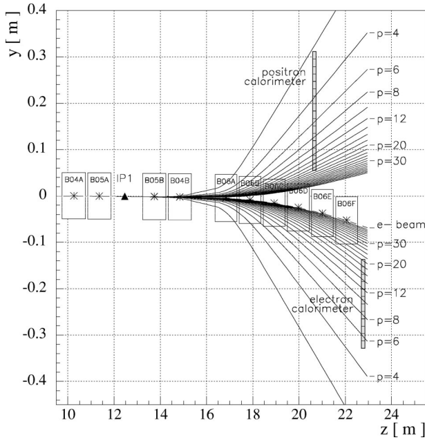
FIG. 16. Calculated trajectories of electrons and positrons of different momenta through the magnetic spectrometer. The location of two calorimeters is shown as well.
