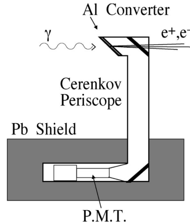
FIG. 23. The forward photon monitor CCM1.
