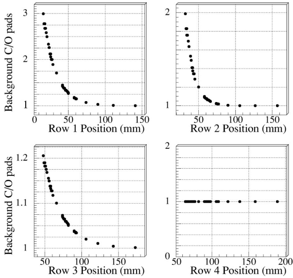
FIG. 56. The “splash” coefficients L_{ii} as functions of the ECAL vertical position.
