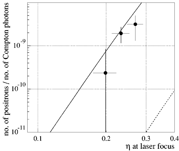
FIG. 48. The subtracted laser-on positron rate for 49.1 GeV beam electrons, normalized to the number of the linear Compton photons. The prediction of the simulation is represented by the solid line. The dashed line indicates the results of the simulation of the trident process.
