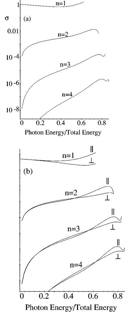
FIG. 5. Calculated spectra, \sigma \equiv (\omega \mathcal{E} / \pi r_0^2 m^2) (dW_n / d\omega') , of backscattered photons produced in the interaction of a 46.6 GeV electron with n=1, 2, 3 , and 4 photons from a linearly polarized 527 nm plane wave with \eta=0.1 , as a function of the ratio \omega'/\mathcal{E} of the energy of the backscattered photon to that of the beam energy. (a) Spectra summed over the polarization of the backscattered photon. (b) Spectra for polarization of the backscattered photon parallel and perpendicular to that of the incident wave.
