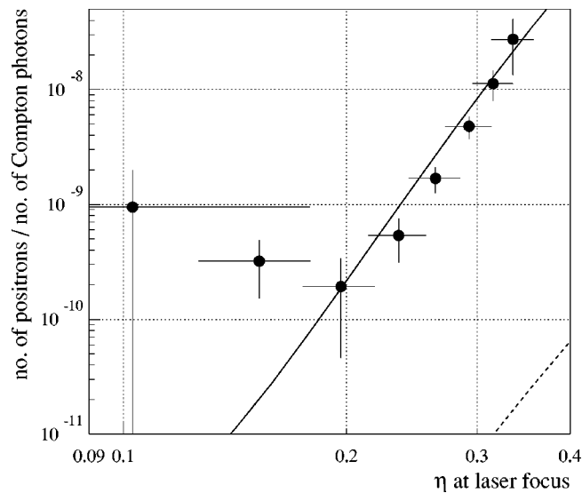
FIG. 46. The dependence of the positron rate on the laser field-strength parameter \eta when the rate is divided by the number of Compton scatters inferred from the EC37 monitor. The solid line is the prediction per Compton photon based the simulation of the two-step Breit-Wheeler process (1) followed by (2). The dashed line represents the simulation for the one-step trident process (53).
