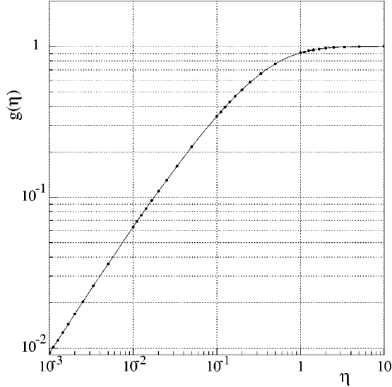
FIG. 9. The function g(\eta) defined by Eq. (51).
