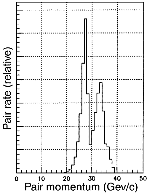
FIG. 43. The relative rate of pair creation by the two-step process of reactions (1),(2) as a function of the total momentum of the pair, according to the simulation of the experiment. The peaks near 27 and 34 GeV/c are due to high-energy photons from n=1 and 2 Compton scattering, respectively.
