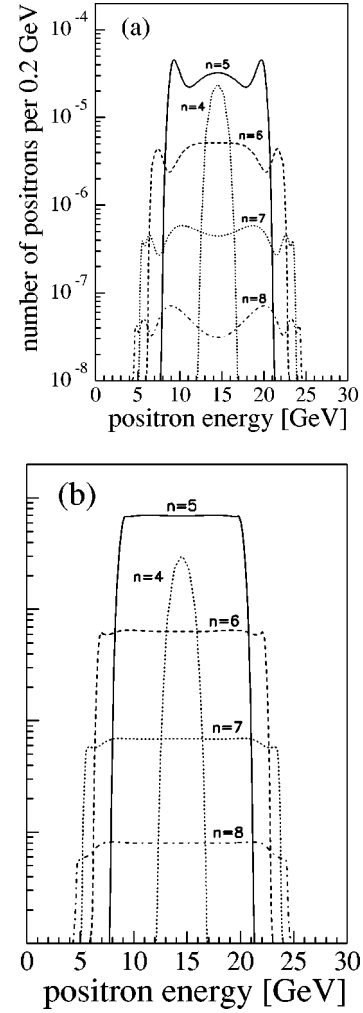
FIG. 8. Calculated energy spectra of positrons produced in the interaction of a 30 GeV photon with a 527 nm laser beam. (a) Parallel polarization. (b) Perpendicular polarization. The curves are labeled by the number of laser photons involved.
