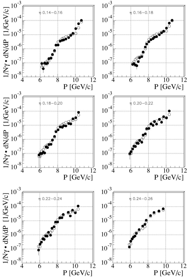
FIG. 38. The scattered electron yield (1/N_\gamma)(dN/dP) , as a function of electron momentum, for 46.6-GeV incident electrons and linearly polarized green laser. The solid dots are the data, and the open circles are the prediction of the simulation. Data are shown for six intervals of the laser field-strength parameter \eta .
