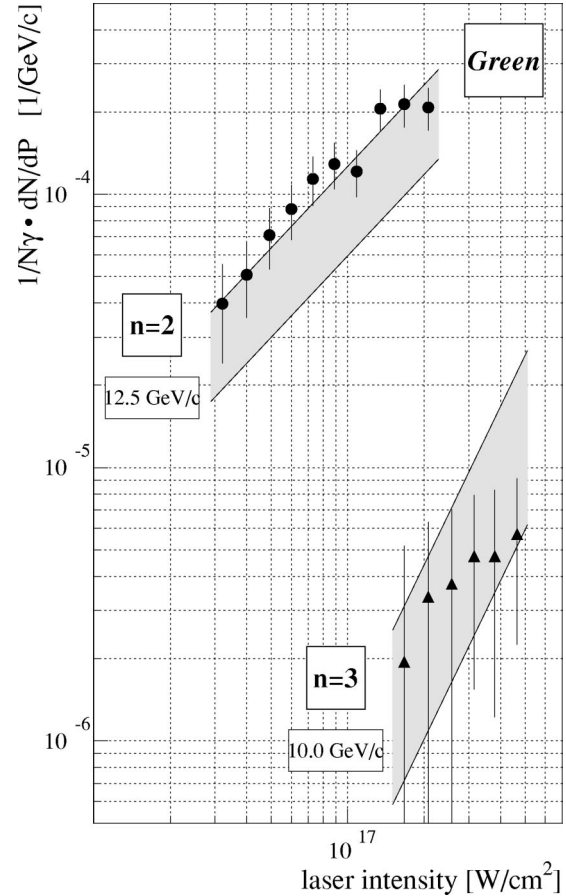
FIG. 36. The scattered electron yield (1/N_\gamma)(dN/dP) vs green laser intensity for two representative electron momenta. The solid circles and triangle are data for which the n=2 and n=3 nonlinear Compton processes dominate, respectively. The simulation for each data set is shown as bands, including the +50\% -30\% uncertainty in the laser intensity.
