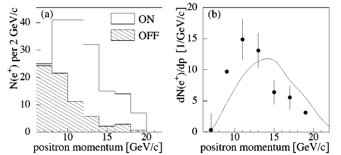
FIG. 42. Number of positron candidates vs momentum for laser-on (ON) and laser-off (OFF) electron pulses. (b) Spectrum of signal positrons obtained by subtracting the laser-off from the laser-on distribution. The curve shows the expected momentum spectrum from the model calculation.
