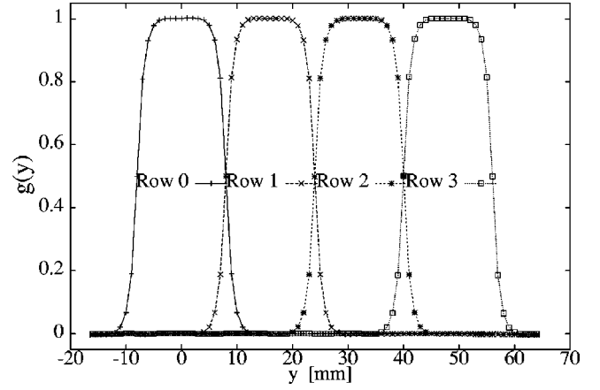
FIG. 57. The aperture functions defined by Eq. (B23) for the top four rows of ECAL.
