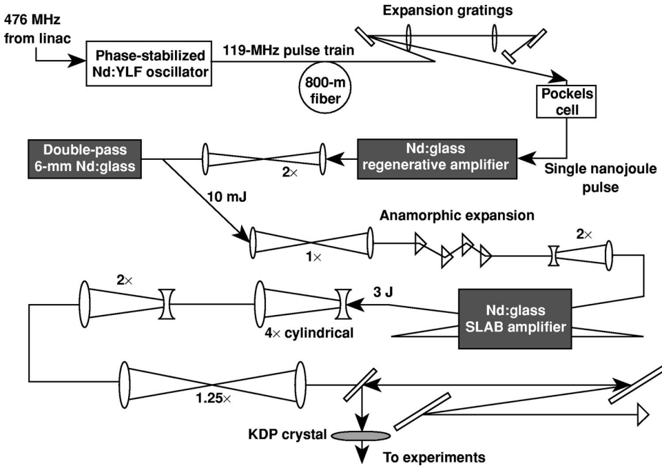
FIG. 12. Schematic of the laser system.
