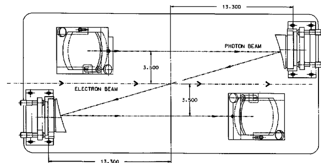
FIG. 13. The optical elements in the interaction point enclosure (IP vacuum box). Dimensions are in inches.
