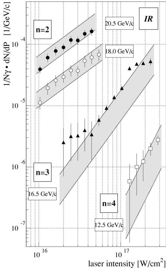
FIG. 35. The scattered electron yield (1/N_\gamma)(dN/dP) vs IR laser intensity for four representative electron momenta. The solid and open circles are data for momenta at which the n=2 Compton process dominate. The triangles and open squares are data for momenta at which the n=3 and n=4 processes dominate, respectively. The simulation for each data set is shown as bands representing the 30% uncertainty in the IR laser intensity. The slopes of the bands are characteristic of the order of the nonlinear process.
