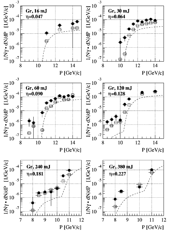
FIG. 34. The yield of nonlinearly scattered electrons, (1/N_\gamma)(dN/dP) vs momentum P , for six different circularly polarized green laser energies. The data are the solid circles with vertical error bars corresponding to the statistical and reconstruction errors added in quadrature. The open boxes are the simulation, with error estimates indicated by the horizontal and vertical lines. The effect of systematic uncertainty in the laser intensity is not shown. The dashed line is the simulation of n=m plural scattering.
