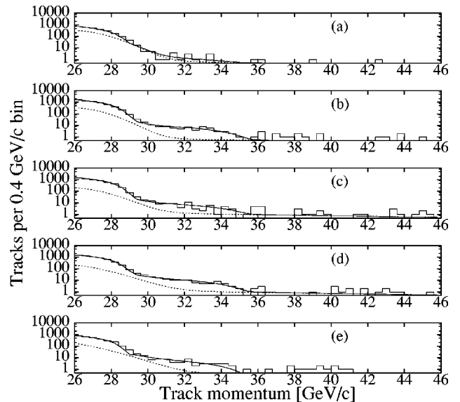
FIG. 40. Single-particle momentum spectra from five subsets of the photon-conversion data.
