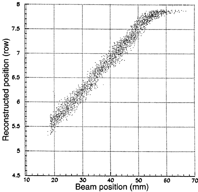
FIG. 19. The reconstructed position of 17.6-GeV electrons incident on the PCAL, in units of the 16-mm-wide rows, as a function of the incident position in mm.
