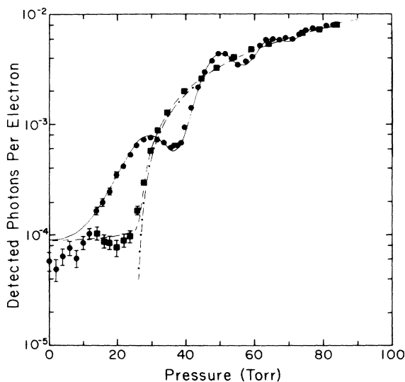
FIG. 2. The number of photons detected per 344-MeV electron. The circles (squares) represent data collected with a magnetic field of 51.3 (0) G. The Polaroid filter transmitted photons with polarization perpendicular to the direction of magnetic field lines. The three smooth curves are from calculations described in the text.
