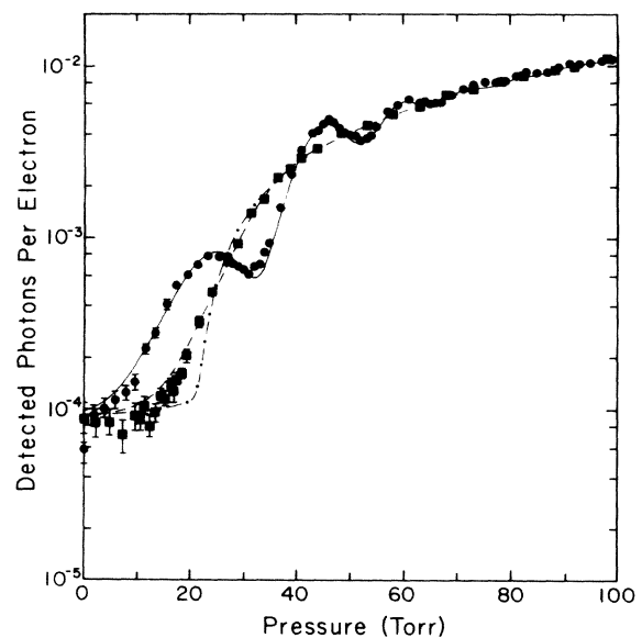
FIG. 3. The number of photons detected per 378-MeV electron. The circles (squares) represent photons with polarization perpendicular (parallel) to the 56.4-G magnetic field. The three smooth curves are from calculations described in the text.
