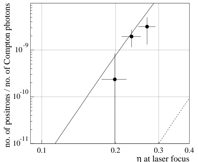
FIG. 48. The subtracted laser-on positron rate for 49.1 GeV beam electrons, normalized to the number of the linear Compton photons. The prediction of the simulation is represented by the solid line. The dashed line indicates the results of the simulation of the trident process.
