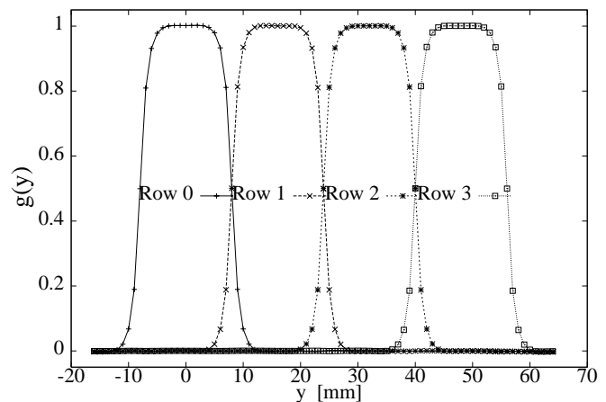
FIG. 57. The aperture functions defined by eq. (107) for the top four rows of ECAL.
