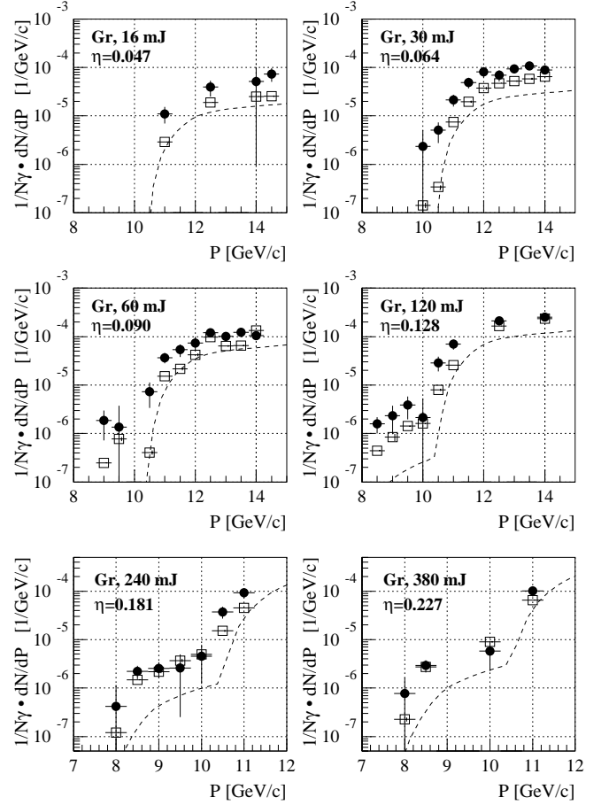
FIG. 34. The yield of nonlinearly scattered electrons, (1/N_\gamma)(dN/dP) vs. momentum P , for six different circularly polarized green laser energies. The data are the solid circles with vertical error bars corresponding to the statistical and reconstruction errors added in quadrature. The open boxes are the simulation, with error estimates indicated by the horizontal and vertical lines. The effect of systematic uncertainty in the laser intensity is not shown. The dashed line is the simulation of n = m plural scattering.
