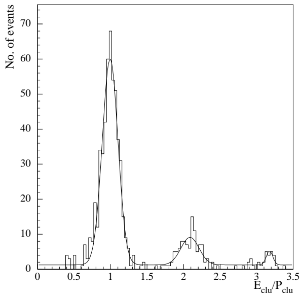
FIG. 32. Distribution of the ratio E_{\text{clu}}/P_{\text{clu}} for calibration clusters in PCAL row 7, which spans momenta from 20.3 to 21.5 GeV.
