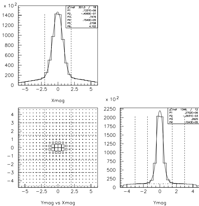
FIG. 30. The two-dimensional distribution of the track positions at the center plane of the 5D36 magnet; the box size is proportional to number of tracks in the bin. Projections on the two transverse axes are also shown. Distances are in mm.
