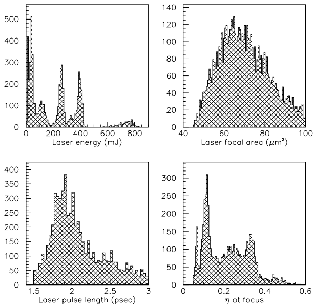
FIG. 28. Laser parameters for all data taken with IR pulses. The value of \eta at the laser focus was calculated by the direct method described in the text.
