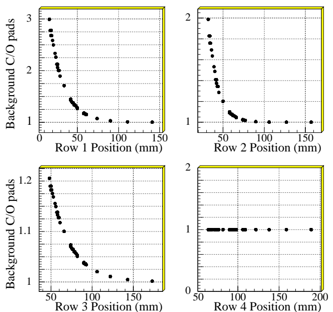
FIG. 56. The “splash” coefficients L_{ii} as function of ECAL vertical position.
