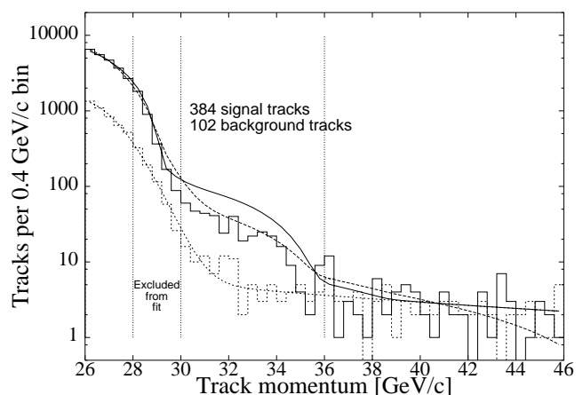
FIG. 39. The momentum spectrum of electrons and positrons from conversion of forward photons into pairs (solid histogram), and the background as estimated from sidebands (dotted histogram). The dotted curve is a fit to the background. The solid and dashed curves are simulations, including the fitted background, in which the value of \eta is taken from the indirect method, or fit to the present data, respectively.
