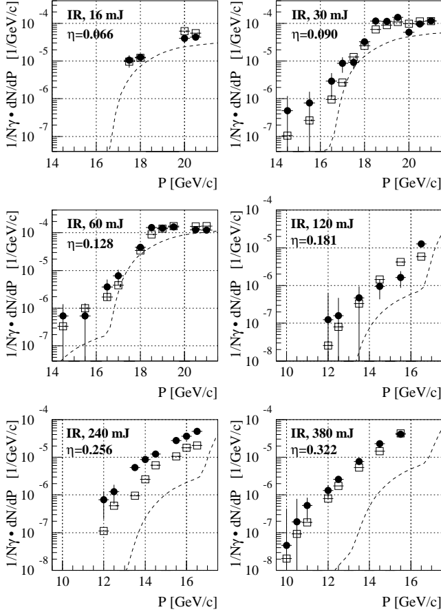
FIG. 33. The yield of nonlinearly scattered electrons, (1/N_\gamma)(dN/dP) vs. momentum P , for six different circularly polarized IR laser energies. The data are the solid circles with vertical error bars corresponding to the statistical and reconstruction errors added in quadrature. The open boxes are the simulation, with error estimates indicated by the horizontal and vertical lines. The effect of systematic uncertainty in the laser intensity is not shown. The dashed line is the simulation of n = m plural scattering.
