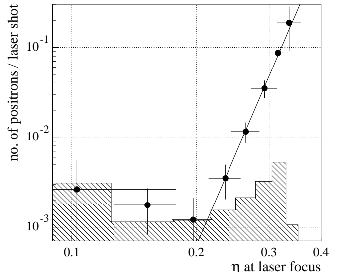
FIG. 44. The dependence of the positron rate per laser shot on the laser field-strength parameter \eta . The line shows a power law fit to the data. The shaded distribution is the 95% confidence limit on the residual background from showers of lost beam particles after subtracting the laser-off positron rate.
