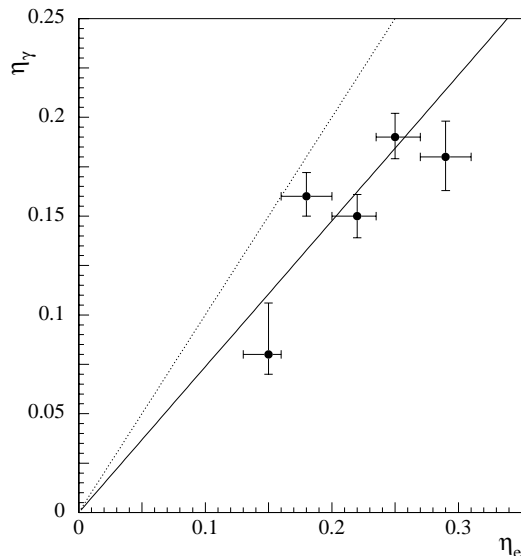
FIG. 41. Photon-based \eta_\gamma vs. the mean value of the nonlinear-electron-based \eta_e for each of the five CCD data subsets. The vertical error bars are from the fit for \eta_\gamma using CCD data, and the horizontal error bars are the rms of the distribution of the monitor \eta_e .
