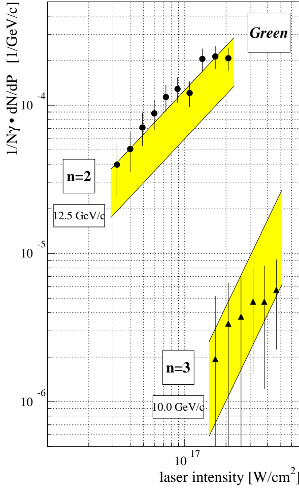
FIG. 36. The scattered electron yield, (1/N_\gamma)(dN/dP) , vs. green laser intensity for two representative electron momenta. The solid circles and triangle are data for which the n = 2 and n = 3 nonlinear Compton processes dominate, respectively. The simulation for each data set is shown as bands, including the +50\% -30\% uncertainty in the laser intensity.
