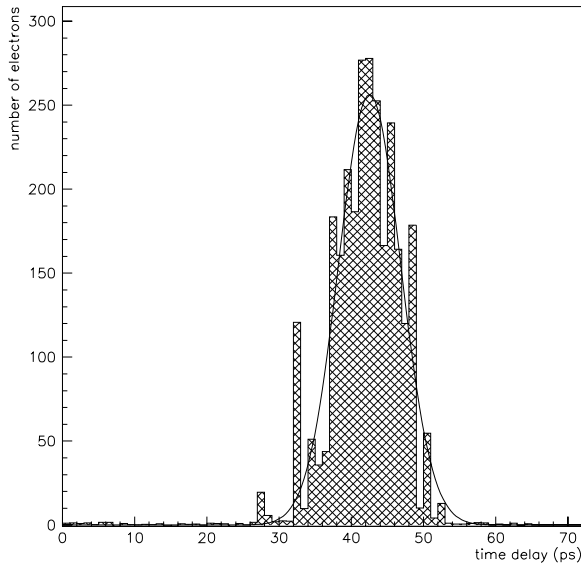
FIG. 15. A “timing curve” showing the number of electrons scattered into the top row of the electron calorimeter as a function of delay of the optical pulse. The standard deviation is \sigma = 4.3 ps.
