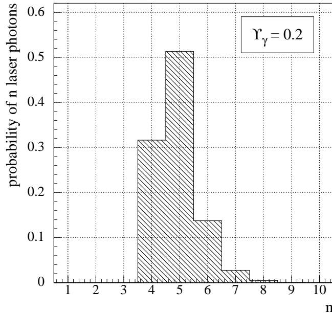
FIG. 45. Calculated probability distribution of the number n of photons absorbed from the laser field in the second step of the two-step Breit-Wheeler pair creation process. Field intensity corresponding to \Upsilon_\gamma = 0.2 ( \eta = 0.4 ) at the laser focus was used for the simulation.
