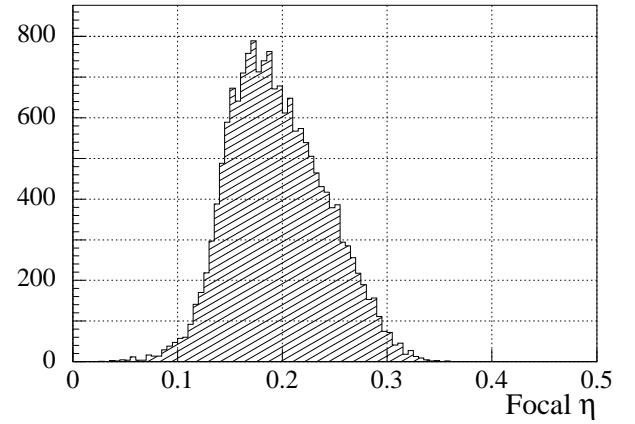
FIG. 37. Distribution of the laser field-strength parameter \eta calculated using the constrained fit (67) for the 46.6 GeV data with linearly polarized green light.
