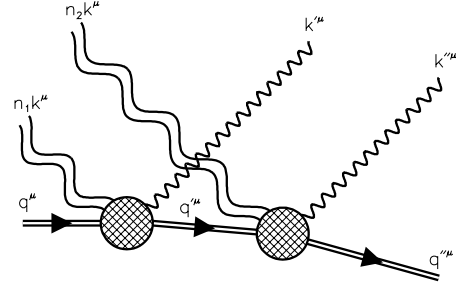
FIG. 7. Plural Compton scattering, (38), of an electron in the laser field with n = n_1 + n_2 and m = 2 . The electron with initial momentum q scatters from n_1 laser photons, emitting a photon with momentum k' , and recoiling with momentum q' ; then the electron scatters again from the laser field, absorbing n_2 laser photons, emitting another photon k'' , and recoiling with momentum q'' .
