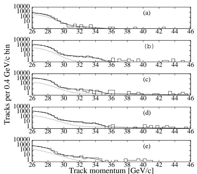
FIG. 40. Single-particle momentum spectra from five subsets of the photon-conversion data.
