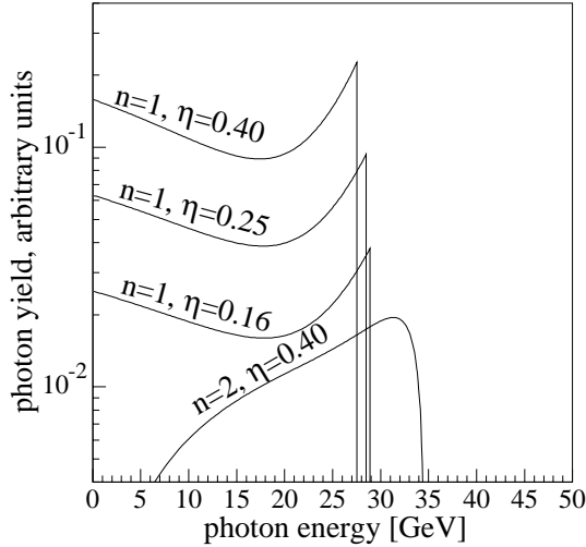
FIG. 2. The calculated rate for nonlinear Compton scattering of 46.6 GeV electrons and 527 nm photons for several values of the field strength parameter \eta , as a function of the energy of the scattered photon.
