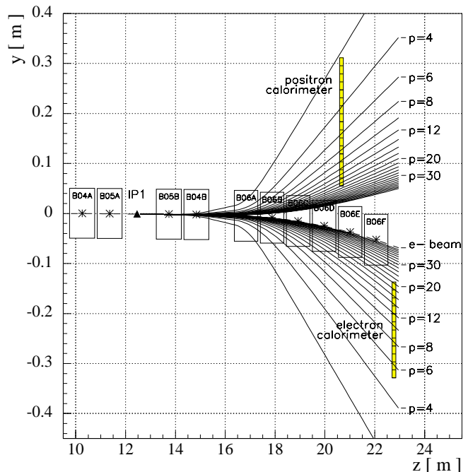
FIG. 16. Calculated trajectories of electrons and positrons of different momenta through the magnetic spectrometer. The location of two calorimeters is shown as well.
