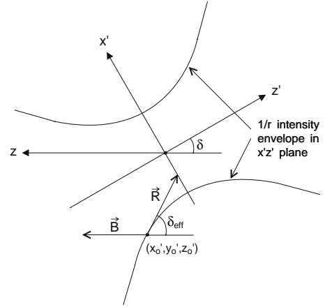
FIG. 51. Effective crossing angle between the laser photons propagating along \vec{R} and the electron beam moving along \vec{B} at the interaction point (x'_0, y'_0, z'_0) .
