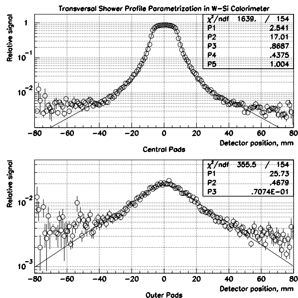
FIG. 55. Top: the response function X_I(\Delta y) for inner columns of the ECAL, summed over longitudinal segments 1-3. Bottom: the function X_O(\Delta y) for outer columns. Circles = data; curve = calculation based on eq. (90).
