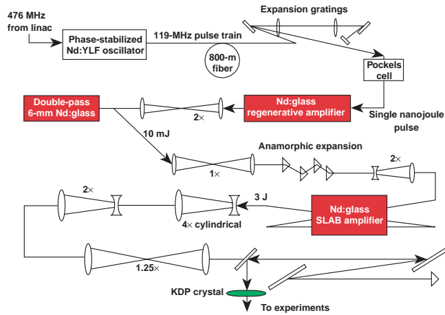
FIG. 12. Schematic of the laser system.
