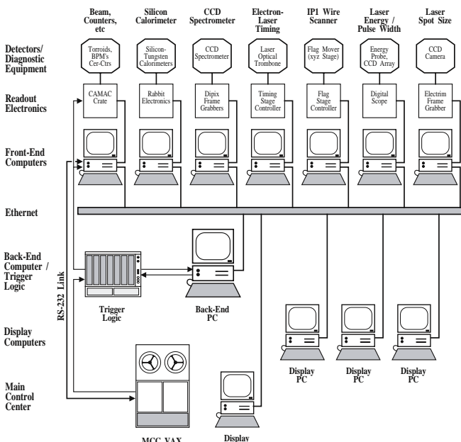
FIG. 25. Components of the data acquisition system.
