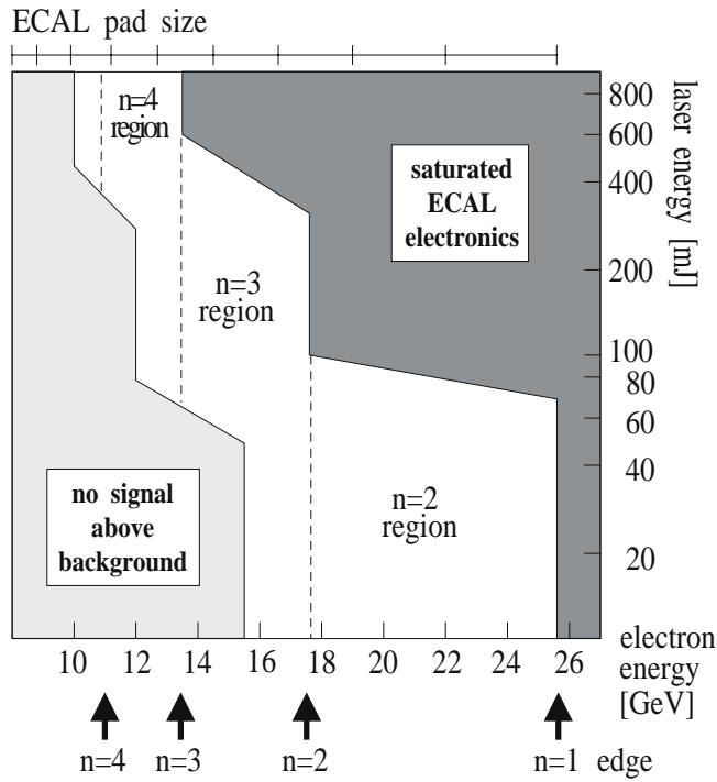
FIG. 26. Portion of recoil electron spectrum accessible to the ECAL for different particle energies and laser energies for IR pulses. The acceptance of a single ECAL tower is shown at the top.
