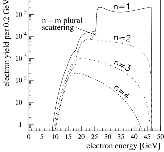
FIG. 4. The calculated rate of scattered electrons for linear, nonlinear and plural Compton scattering for the infrared laser and electron beam parameters given in the text. The solid line is the sum of all possible processes. The rates for n = 2, 3, and 4 nonlinear Compton scattering are shown separately as well.
