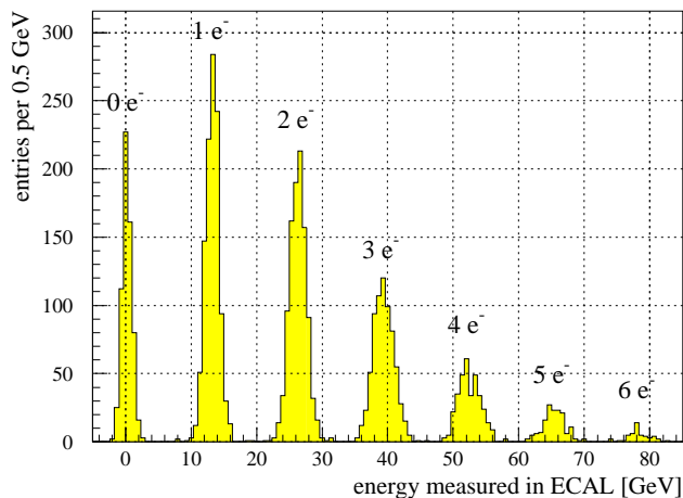
FIG. 18. The response of the ECAL to 13-GeV incident electrons. The peaks due to the simultaneous arrival of up to six electrons are clearly distinguished.
