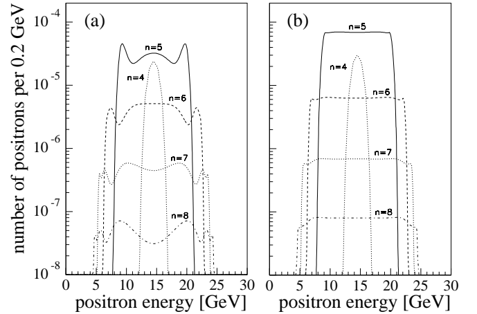
FIG. 8. Calculated energy spectra of positrons produced in the interaction of a 30 GeV photon with a 527 nm laser beam. (a) Parallel polarization. (b) Perpendicular polarization. The curves are labelled by the number of laser photons involved.
