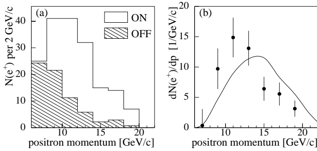
FIG. 42. Number of positron candidates vs. momentum for laser-on (ON) and laser-off (OFF) electron pulses. (b) Spectrum of signal positrons obtained by subtracting the laser-off from the laser-on distribution. The curve shows the expected momentum spectrum from the model calculation.
