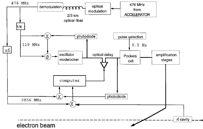
FIG. 14. Diagram of the timing system for the synchronization of the laser pulses with the electron beam.
