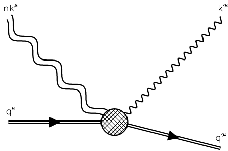
FIG. 6. Representation of nonlinear Compton scattering, (1). An electron with quasimomentum q in a strong field (indicated by a double line) absorbs n photons (indicated by double sinusoids), emits a high-energy photon k' , and recoils with momentum q' .
