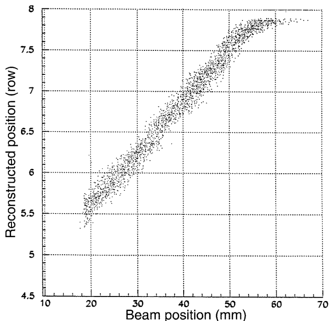
FIG. 19. The reconstructed position of 17.6-GeV electrons incident on the PCAL, in units of the 16-mm-wide rows, as a function of the incident position in mm.
