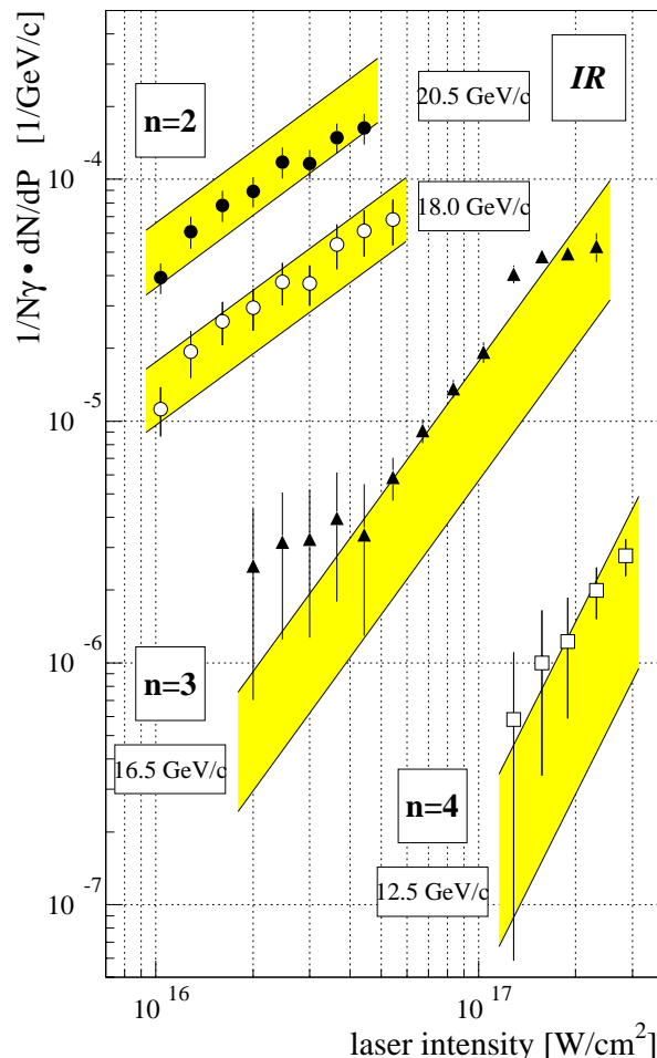
FIG. 35. The scattered electron yield, (1/N_\gamma)(dN/dP) , vs. IR laser intensity for four representative electron momenta. The solid and open circles are data for momenta at which the n = 2 Compton process dominate. The triangles and open squares are data for momenta at which the n = 3 and n = 4 processes dominate, respectively. The simulation for each data set is shown as bands representing the 30% uncertainty in the IR laser intensity. The slopes of the bands are characteristic of the order of the nonlinear process.
