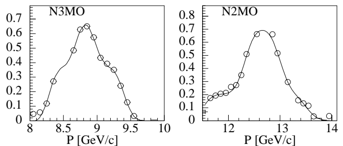
FIG. 24. Measured acceptances of electron detectors N2MO and N3MO vs. electron momentum.
