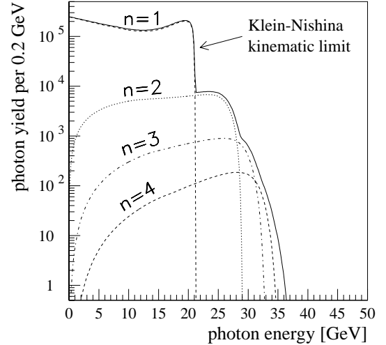
FIG. 3. The calculated rate of scattered photons for nonlinear Compton scattering for the infrared laser and electron beam parameters given in the text. The dashed curves show the rates for n = 1, 2, 3 , and 4 nonlinear Compton scattering. The solid curve is the sum of all orders.
