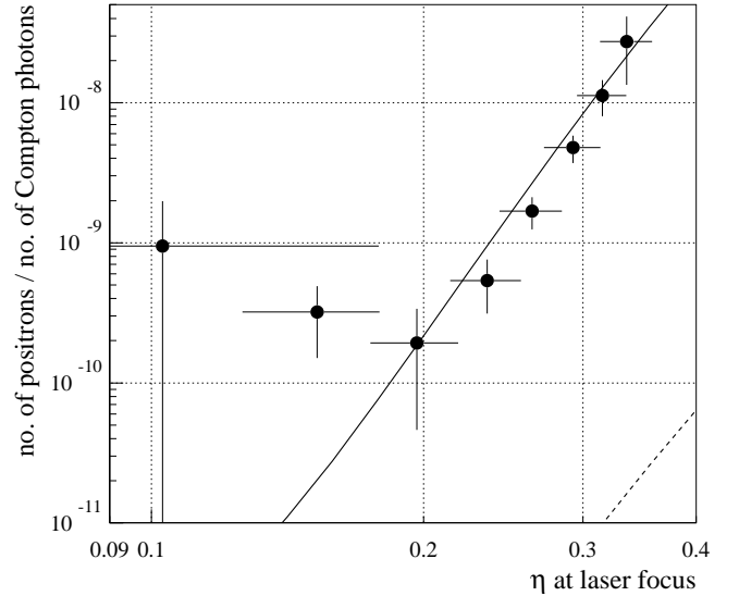
FIG. 46. The dependence of the positron rate on the laser field-strength parameter \eta when the rate is divided by the number of Compton scatters inferred from the EC37 monitor. The solid line is the prediction per Compton photon based the simulation of the two-step Breit-Wheeler process, (1) followed by (2). The dashed line represents the simulation for the one-step trident process (53).
