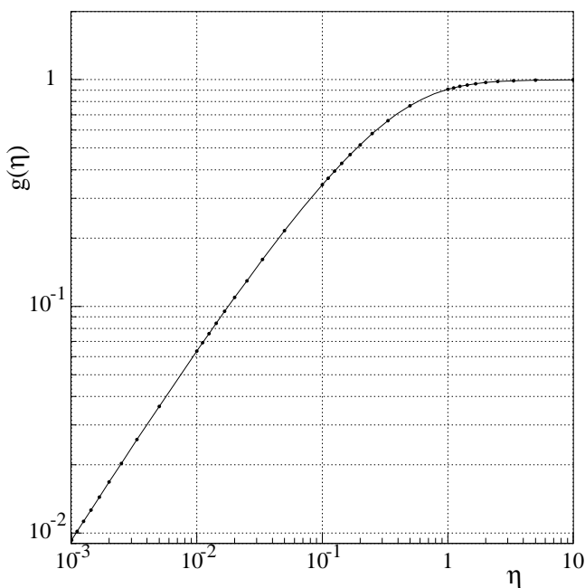
FIG. 9. The function g(\eta) defined by eq. (51).
