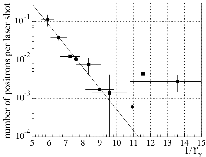
FIG. 49. Number of positrons per laser shot as a function of 1/\Upsilon_\gamma . The circles are the 46.6 GeV data whereas the squares are the 49.1 GeV data. The solid line is a fit to the data.
