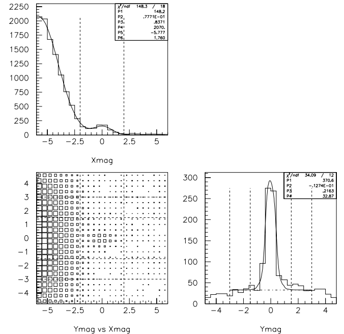
FIG. 31. The distribution of the track positions at the center plane of the magnet, using only high momentum electron tracks. Distances are in mm.
