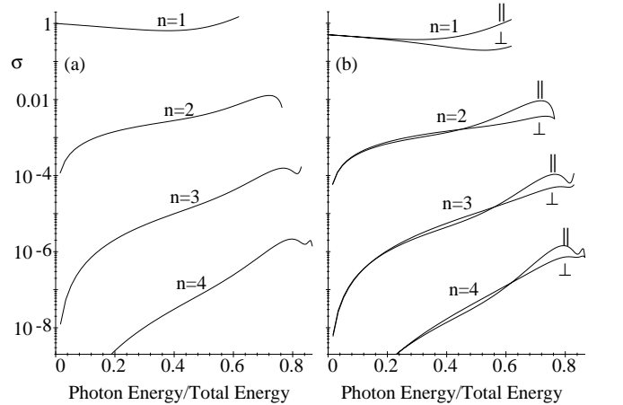
FIG. 5. Calculated spectra, \sigma \equiv (\omega \mathcal{E} / \pi r_0^2 m^2) (dW_n / d\omega') , of backscattered photons produced in the interaction of a 46.6 GeV electron with n = 1, 2, 3, and 4 photons from a linearly polarized 527 nm plane wave with \eta = 0.1 , as a function of the ratio \omega' / \mathcal{E} of the energy of the backscattered photon to that of the beam electron. (a) Spectra summed over the polarization of the backscattered photon. (b) Spectra for polarization of the backscattered photon parallel and perpendicular to that of the incident wave.
