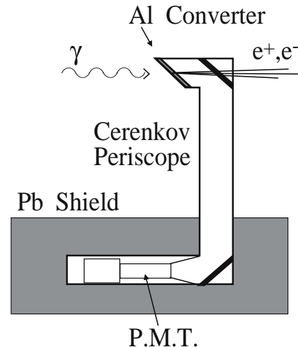
FIG. 23. The forward photon monitor CCM1.
