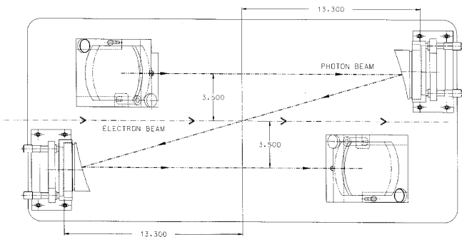
FIG. 13. The optical elements in the interaction point enclosure (IP vacuum box). Dimensions are in inches.
