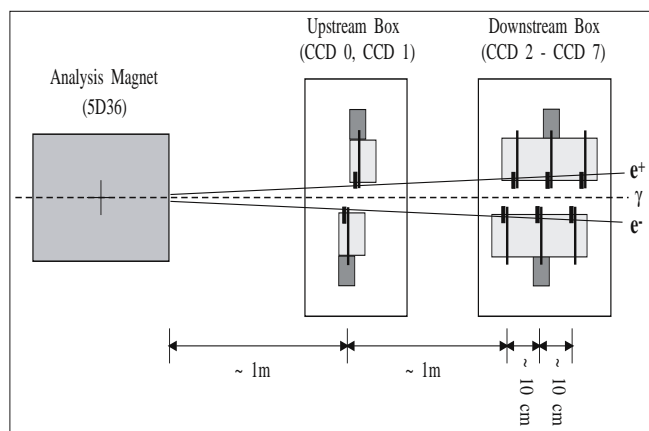
FIG. 22. Schematic of the CCD pair spectrometer.
