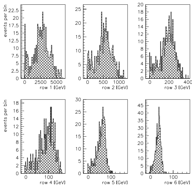
FIG. 29. The ECAL signal for \sim 1600 pulses of IR laser of 400 mJ, with the ECAL positioned to accept electrons with energies less than 15.5 GeV. The energy distribution obtained in the center pads for rows 1-6 is shown, with pedestals and electron-beam-only backgrounds subtracted, but without any other corrections.
