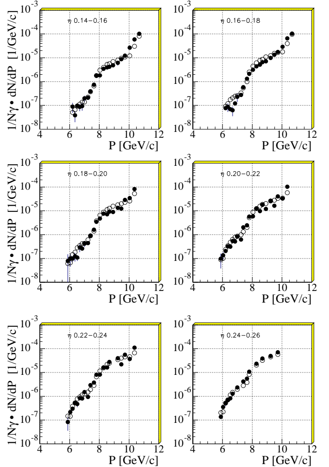
FIG. 38. The scattered electron yield (1/N_\gamma)(dN/dP) , as a function of electron momentum, for 46.6-GeV incident electrons and linearly polarized green laser. The solid dots are the data, and the open circles are the prediction of the simulation. Data are shown for six intervals of the laser field-strength parameter \eta .
