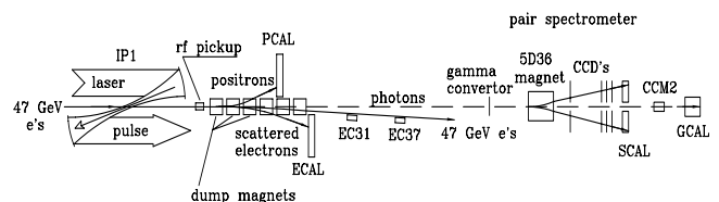
FIG. 11. Schematic of the experimental setup: The laser pulses crossed through the electron beam at the interaction point, IP1. The scattered electrons were deflected by the dump magnets into the electron calorimeter (ECAL). Positrons were deflected into the positron calorimeter (PCAL). The scattered photons were detected in a Čerenkov counter (not shown), or converted to e^+e^- pairs which could be detected by the pair spectrometer.
