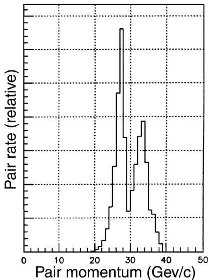
FIG. 43. The relative rate of pair creation by the two-step process of reactions (1-2) as a function of the total momentum of the pair, according to the simulation of the experiment. The peaks near 27 and 34 GeV/c are due to high-energy photons from n = 1 and 2 Compton scattering, respectively.
