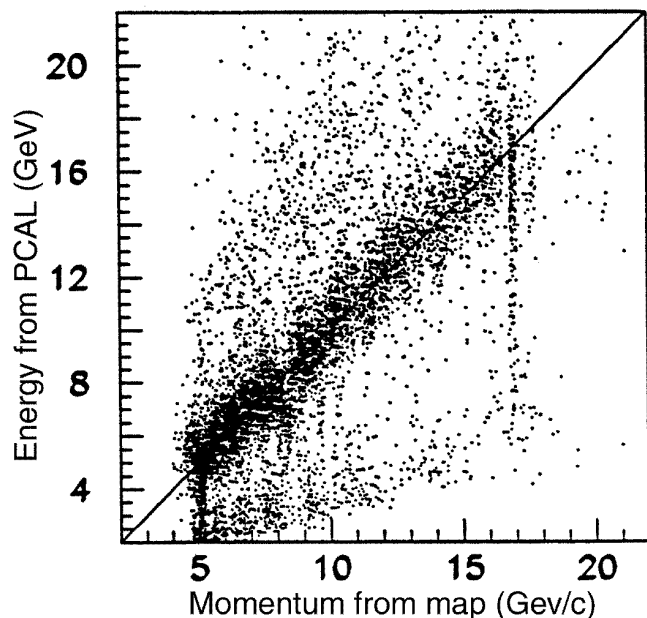
FIG. 21. The energy vs. momentum of positrons observed in the PCAL from a calibration run with a 19-GeV electron beam incident on a foil in IP1.
