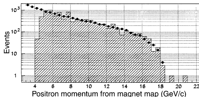
FIG. 20. The observed (histogram) and calculated (points) spectra of positrons detected in the PCAL during a calibration run with 19-GeV electrons and a thin foil inserted at IP1.
