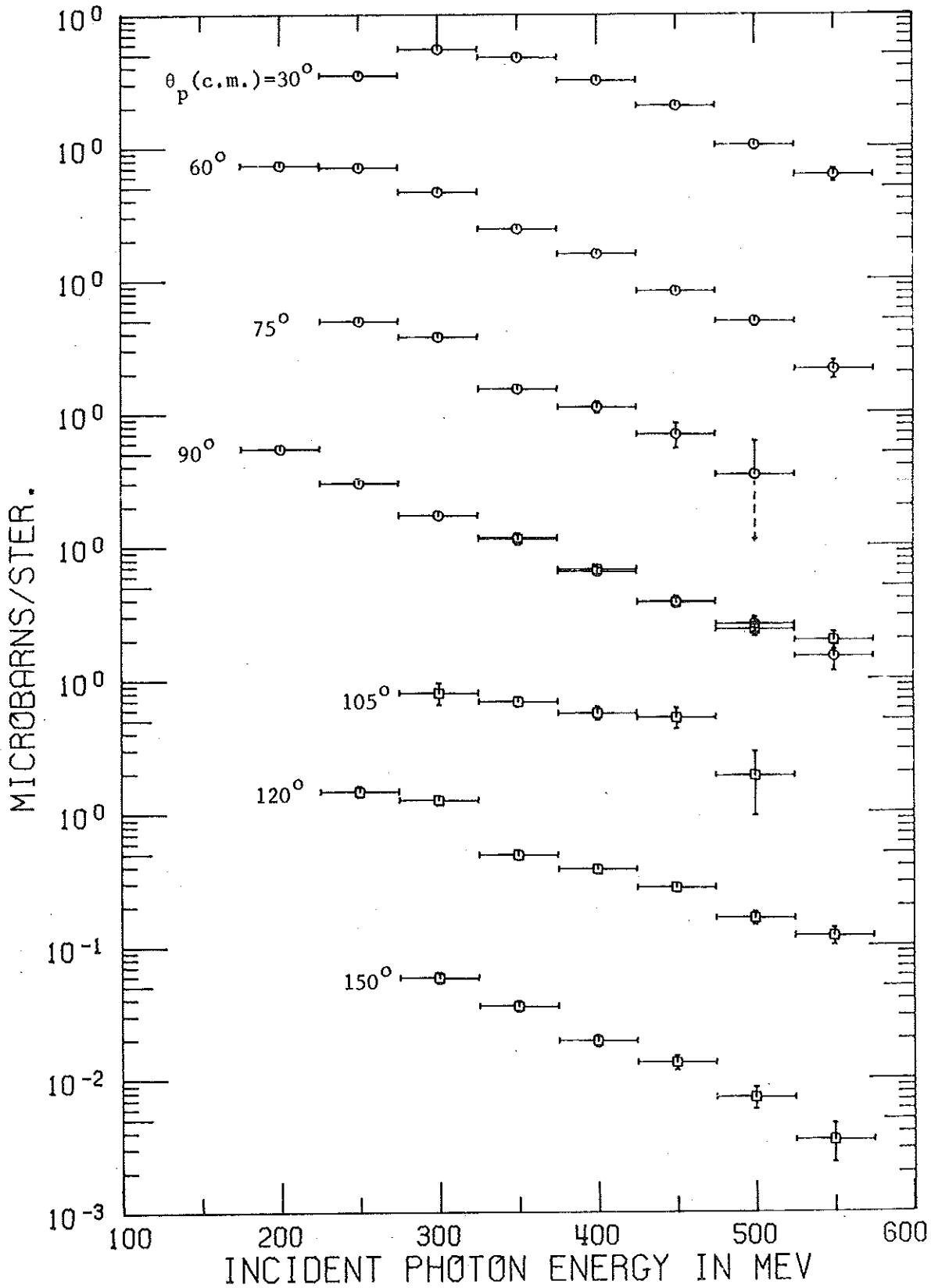
Figure 4.2 He 3 Photodisintegration Differential Cross-Sections in 50 MeV Bins
