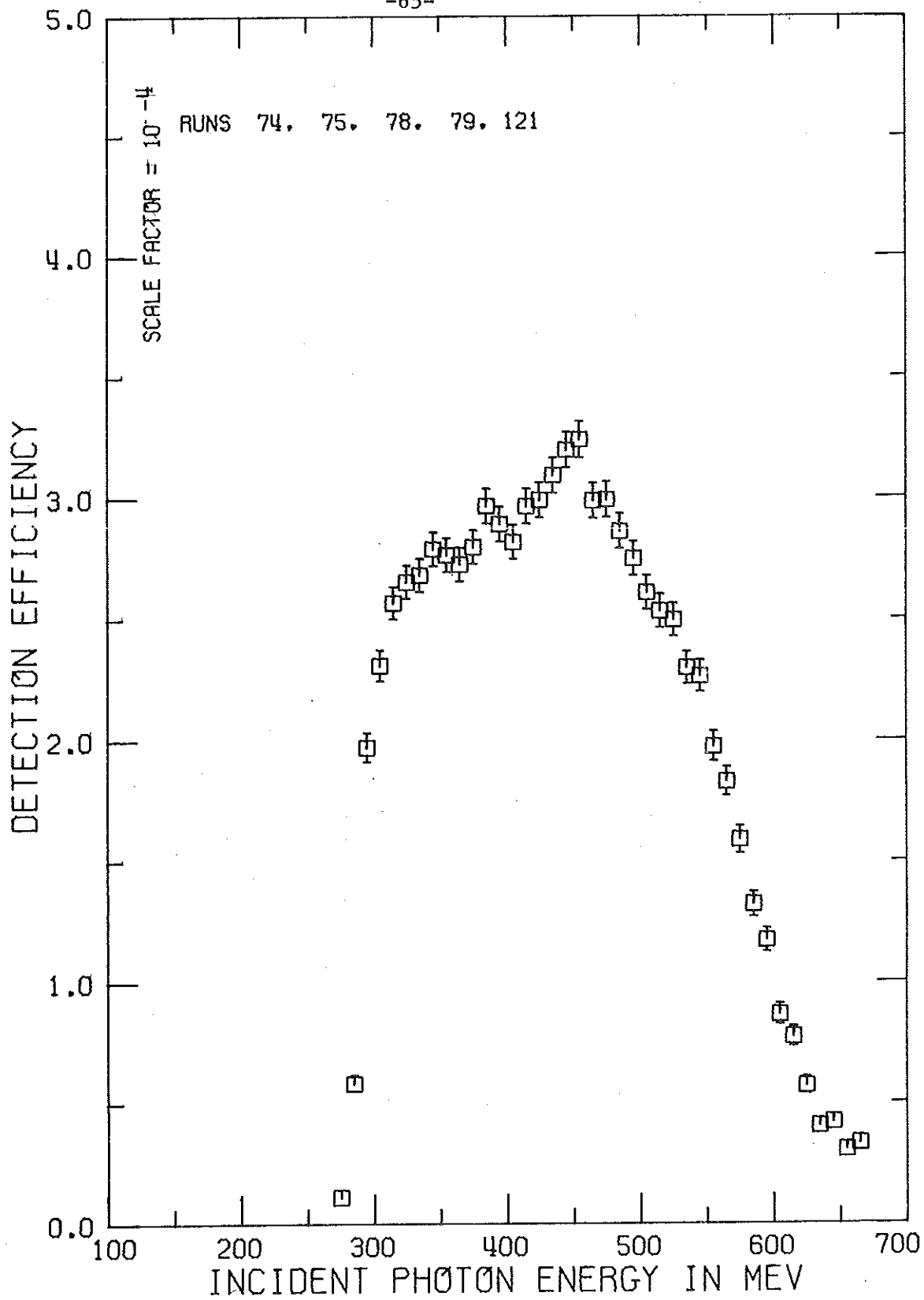
Figure 3.9 Example of the Monte Carlo Efficiency Calculation
