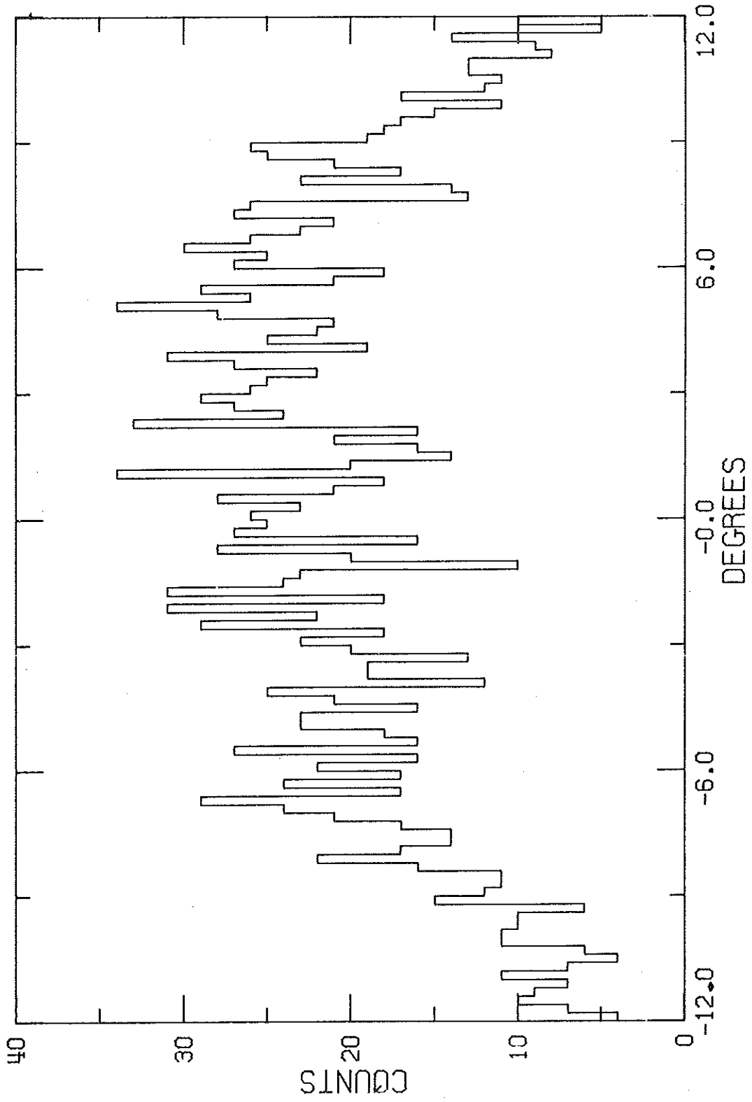
Figure 6.17 The Coplanarity Distribution for Background Events Generated by the Monte Carlo Calculation
