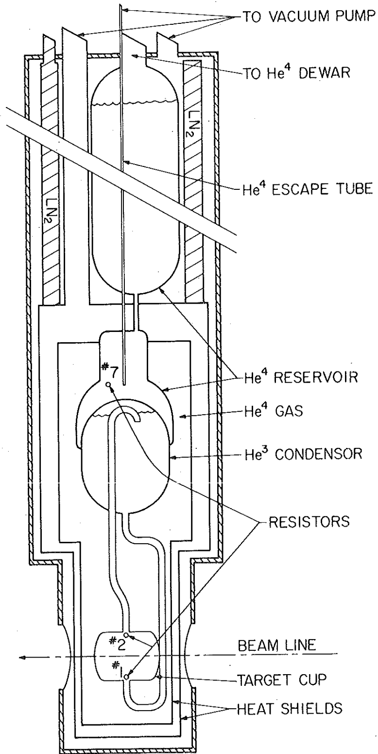
Figure 6.8 The \text{He}^3 Target
