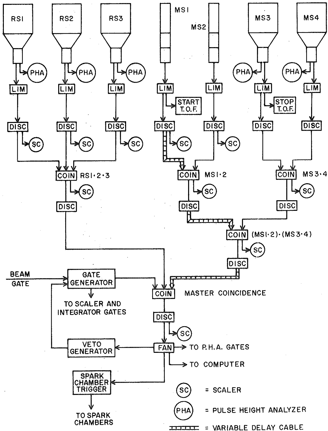
Figure 2.5 The Trigger Electronics
