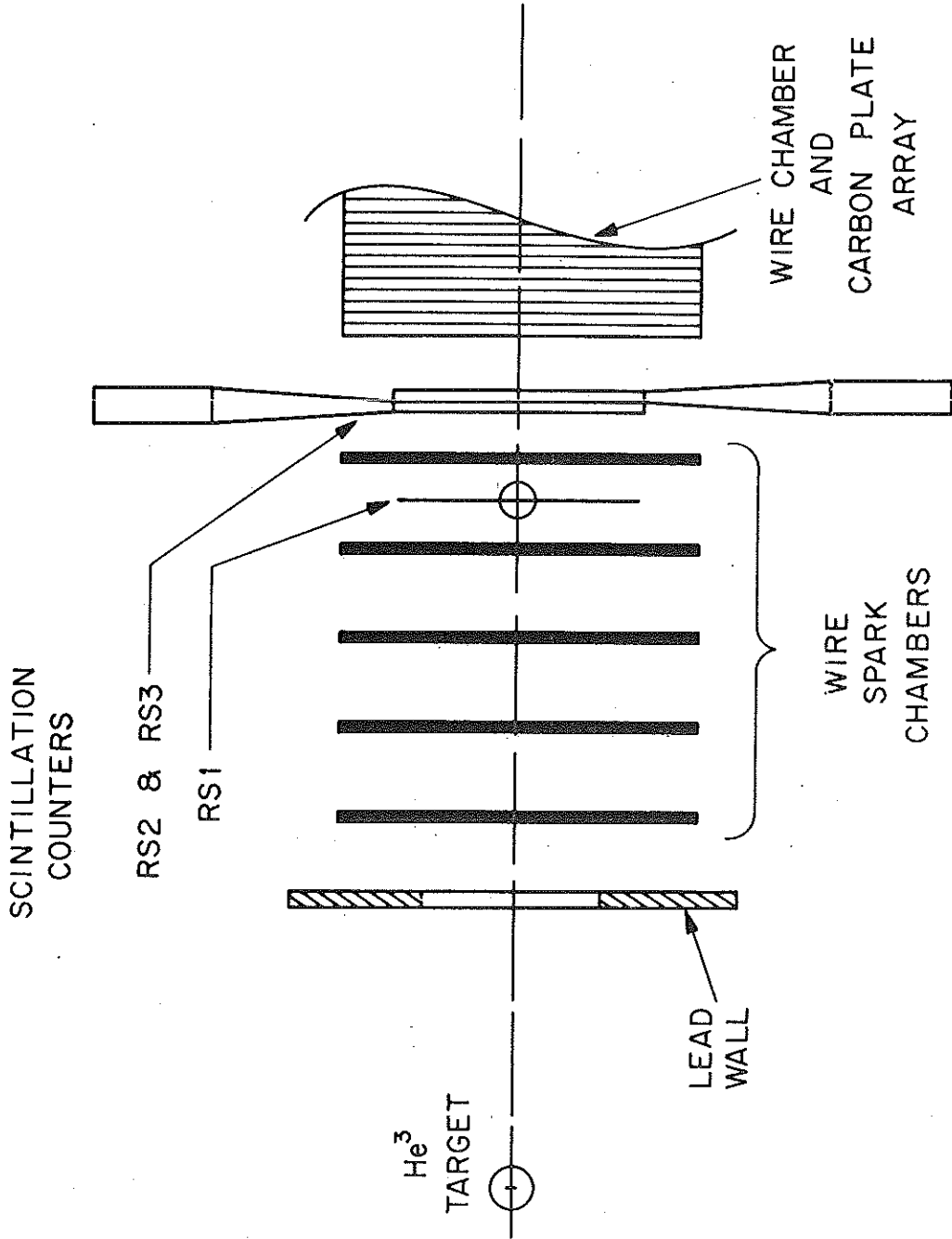
Figure 2.4 The Range Array
