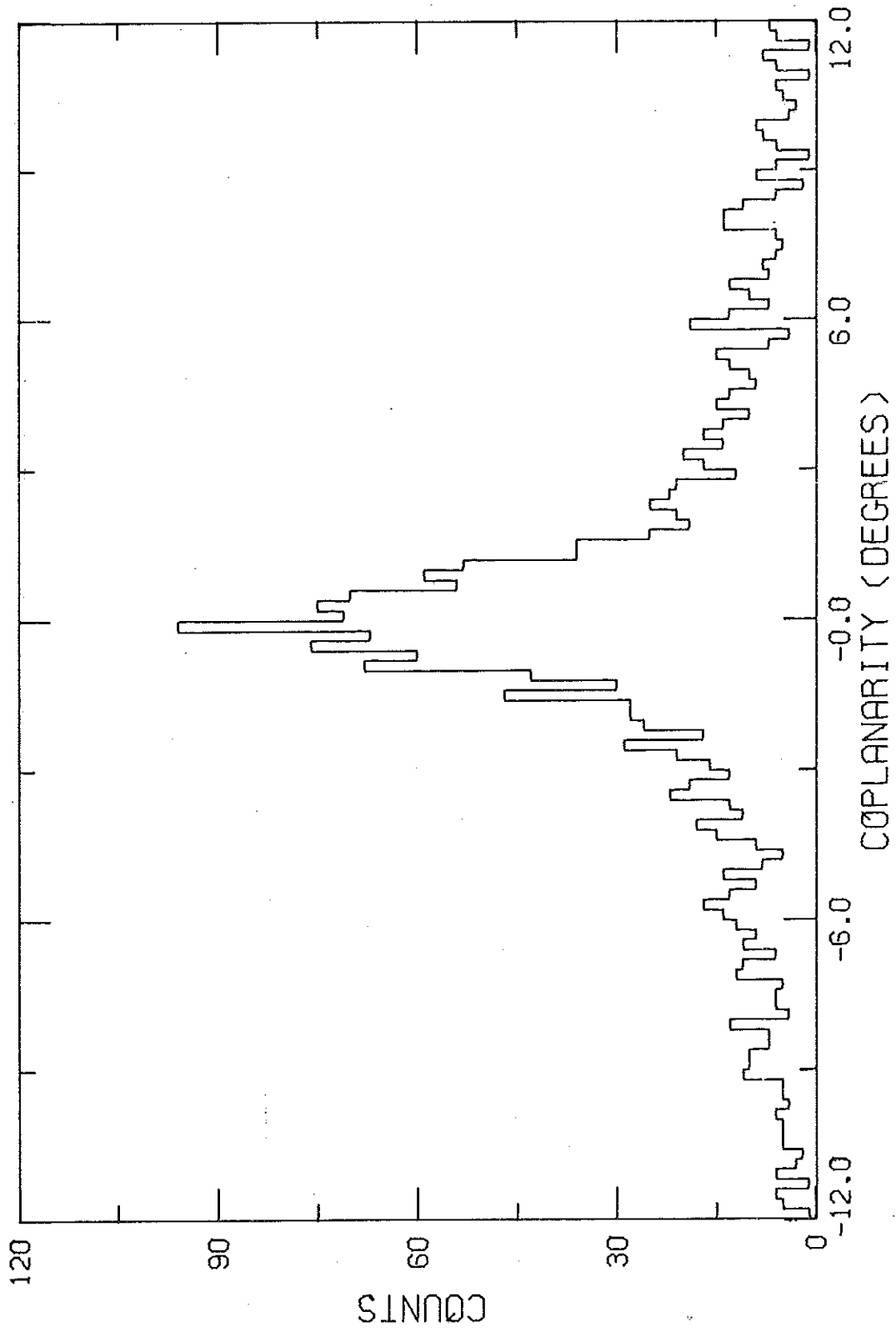
Figure 3.3 A Raw Coplanarity Distribution
