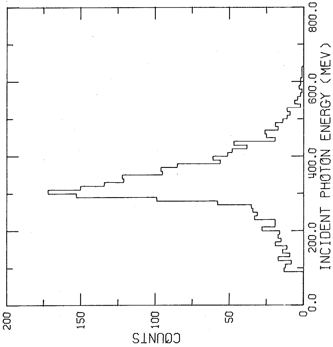
Figure 3.5 A Raw Incident Photon Energy Spectrum
