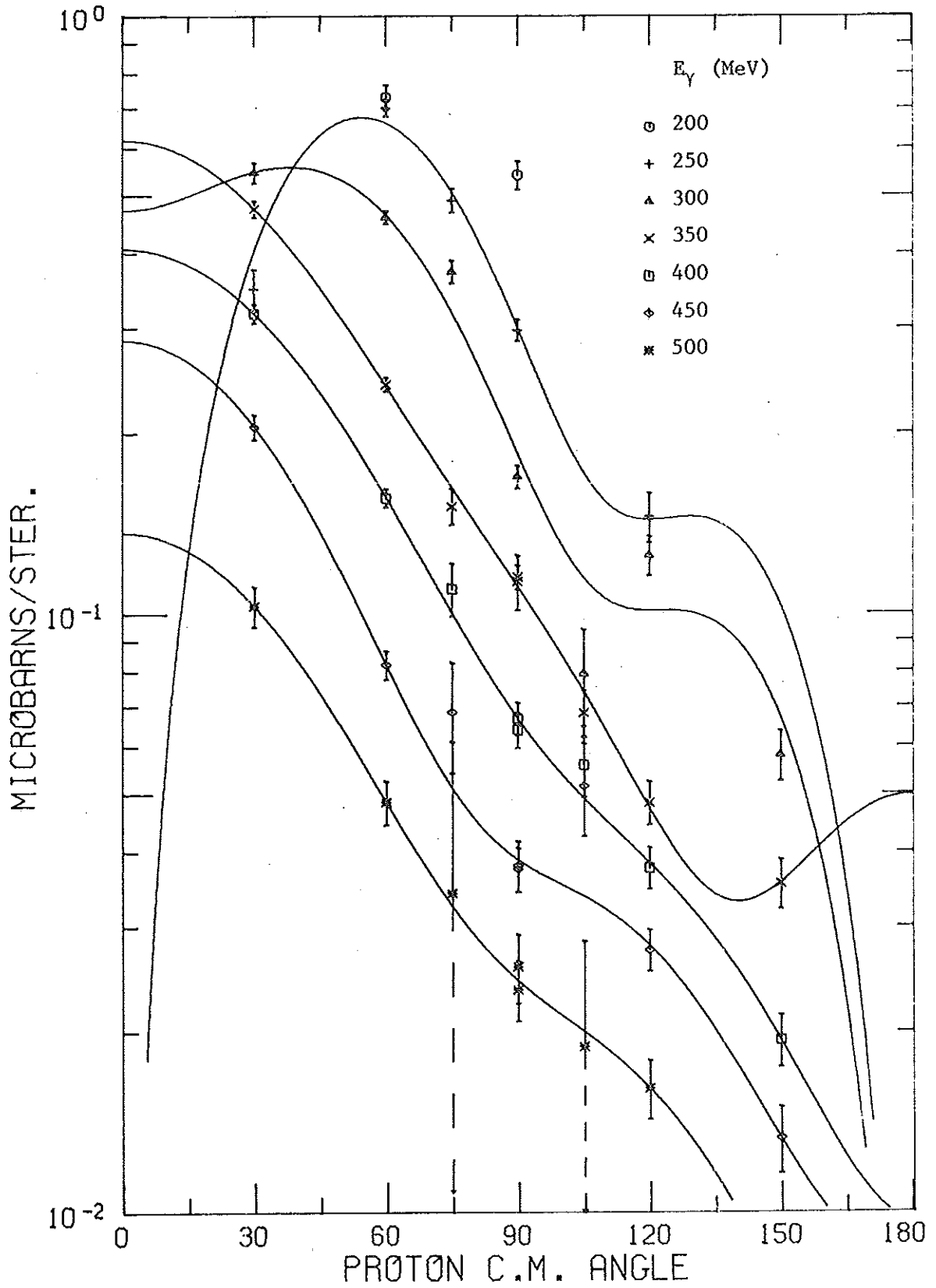
Figure 4.10 Summary of He 3 Photodisintegration Angular Distributions and Fits
