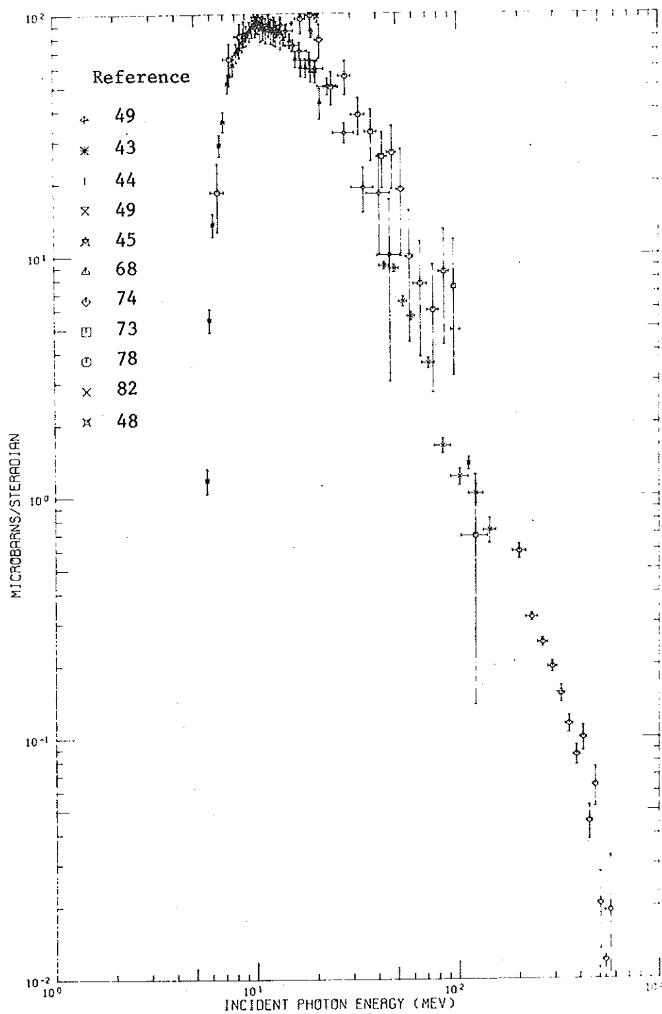
Figure 6.1 Existing Data on \text{He}^3 Photodisintegration Differential Cross-Sections at 90^\circ (c.m.)
