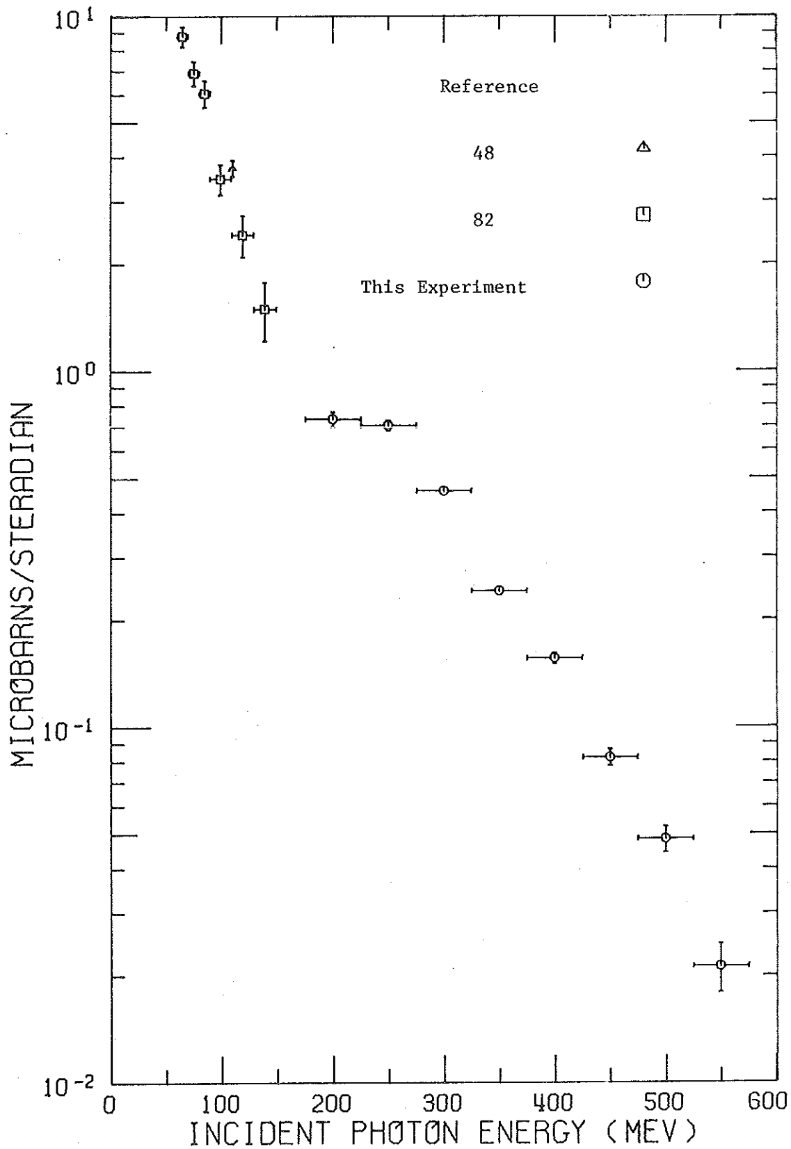
Figure 5.3 Comparison of He 3 Photodisintegration Differential Cross-Section Data at 60°(c.m.)
