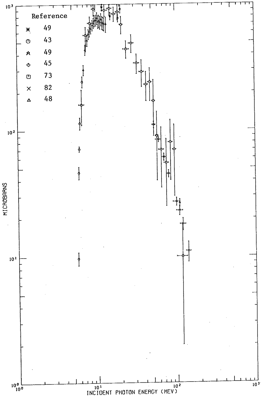
Figure 6.2 Existing Data on He 3 Photodisintegration Total Cross-Sections
