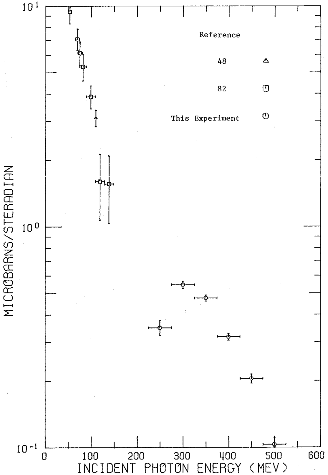
Figure 5.2 Comparison of He 3 Photodisintegration Differential Cross-Section Data at 30° (c.m.)
