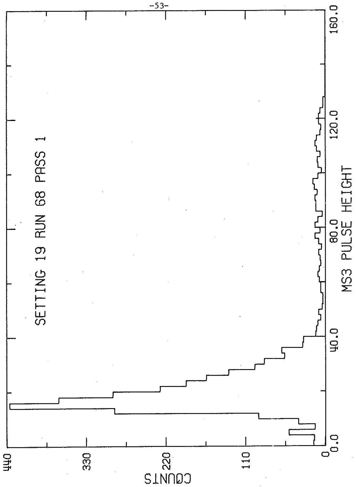
Figure 3.7 A Raw Pulse Height Spectrum in Counter MS3
