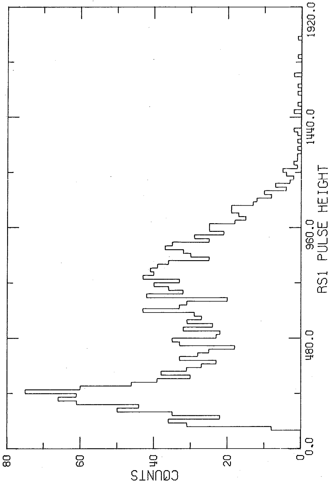
Figure 3.6 A Raw Pulse Height Spectrum in Counter RS1
